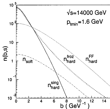
FIG. 8. Soft and hard component of n(b,s) in the three models described in the text.
