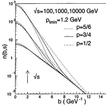
FIG. 7. The average number of collisions for the singular \alpha_s case for different values of the singularity parameter p .
