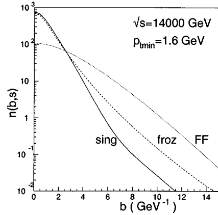
FIG. 9. The average number of collisions in the form factor model and the Bloch-Nordsieck model, at LHC energy.
