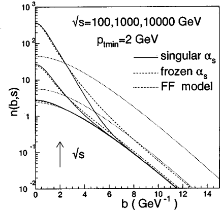
FIG. 6. The average number of collisions for the frozen and singular \alpha_s case in comparison with the FF model at various c.m. energy values.
