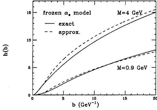
FIG. 12. Comparison between the approximate and the actual numerical integration for h(b, M, \Lambda) for various values for M , in the frozen \alpha_s model.
