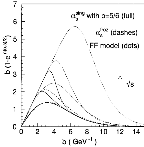
FIG. 10. The integrand of the eikonal formulation for \sigma_{tot} , for p_{tmin}=2 GeV in the three different models described in the text, for a range of c.m. energy values 100,1000,10000 GeV.
