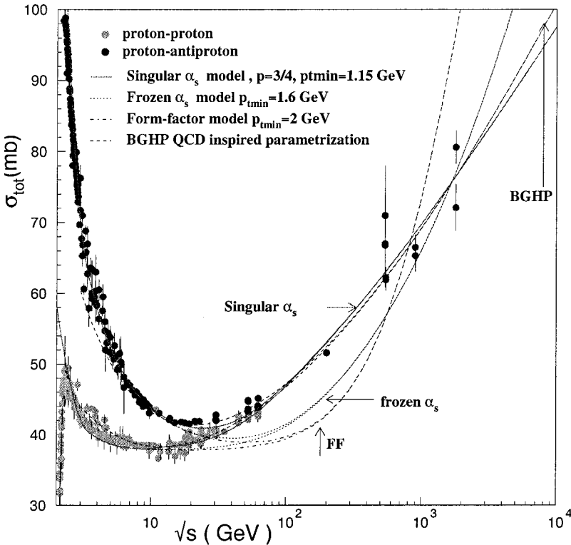
FIG. 11. Total p - p and \bar{p}p cross sections and comparison with various models.
