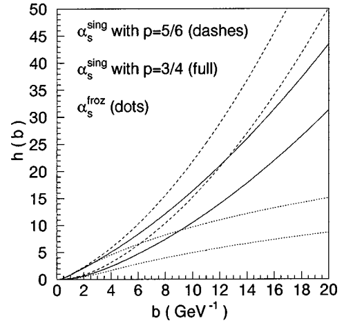
FIG. 3. Comparison between numerically integrated expressions for h(b, M, \Lambda) for singular and frozen \alpha_s . M=1 (lower) and 4 GeV (upper).
