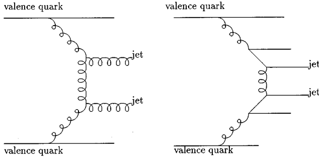
FIG. 1. Two typical subprocesses contributing to the rise of the total proton-proton cross section.
