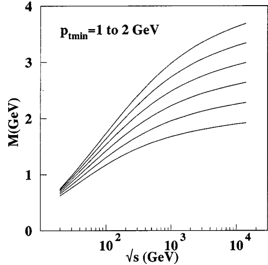
FIG. 2. The maximum value kinematically allowed for the transverse momentum of the single gluon, averaged over densities (GRV-LO parametrization) and for different p_{tmin} values, as a function of the c.m. energy of the colliding protons.
