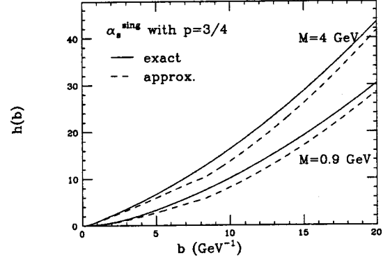
FIG. 13. Comparison between the approximate and the actual numerically computed expression for h(b, M, \Lambda) for the singular \alpha_s model.
