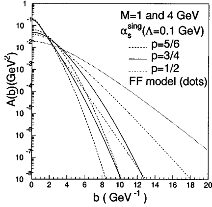
FIG. 5. As in Fig. 4 for singular \alpha_s , for various values of the parameter p .
