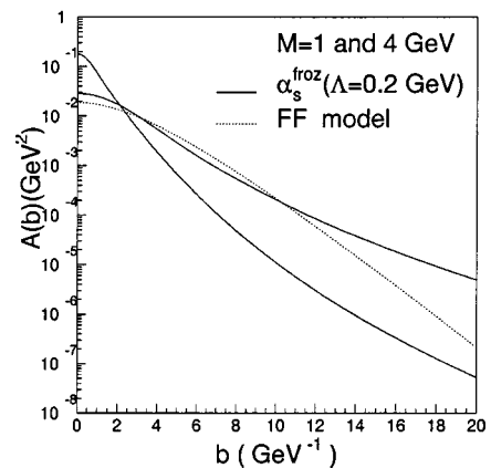
FIG. 4. The overlap function A_{BN}(b) for frozen \alpha_s and comparison with the form factor model.
