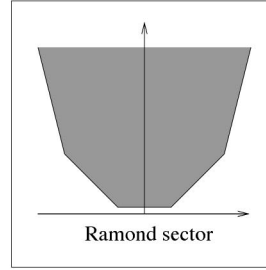
FIG. 5. Allowed region for states belonging to unitary representations of the (NS) superconformal algebra. The dashed curve represents the continuous spectral flow h_\eta = j_\eta^2/k of the point h=j=0 . Spectral flow slides the boundary polygon along the parabola; a half unit of flow gives the Ramond sector (inset).
