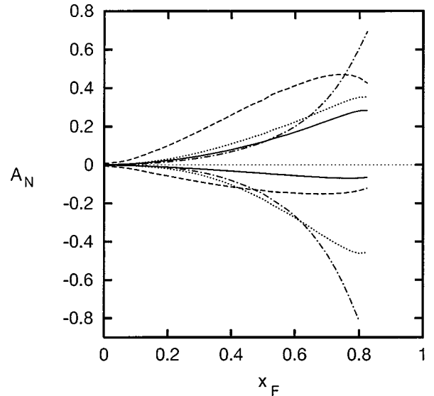
FIG. 6. Single spin asymmetry, as predicted by our model (with Collins effects only), for the production of charged (upper curves) and neutral (lower curves) kaons, (K^+ + K^-)/2 and (K^0 + \bar{K}^0)/2 , respectively. The solid lines correspond to the BKK1 set of unpolarized fragmentation functions [21], the dashed lines correspond to the BKK2 set [23], the dotted lines to the GR set [24], and the dashed-dotted lines to the IMR set [25]; see Ref. [4] and text for further details.
