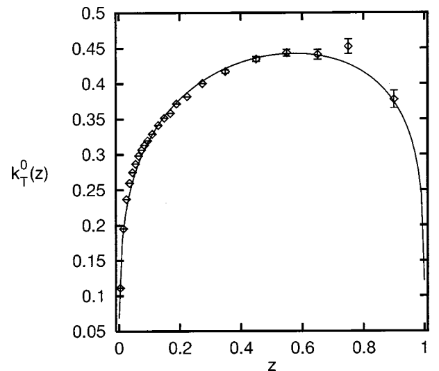
FIG. 1. The pion intrinsic average transverse momentum k_\perp^0 in a jet as a function of z . The diamonds are the data from Abreu et al. [19], the continuous line is our fit, as given by Eq. (17).
