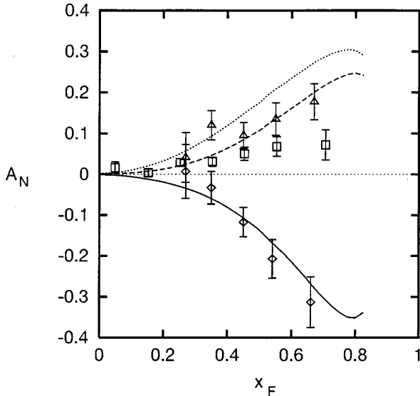
FIG. 5. Single spin asymmetry for pion production in \bar{p}^\uparrow p \rightarrow \pi X . The data points are the E704 experimental single spin asymmetries [22] for \pi^+ (diamonds), \pi^0 (squares), and \pi^- (triangles). The solid line is the result of our model (with Collins effect only) for \pi^+ , the dashed line for \pi^0 , and the dotted line for \pi^- .
