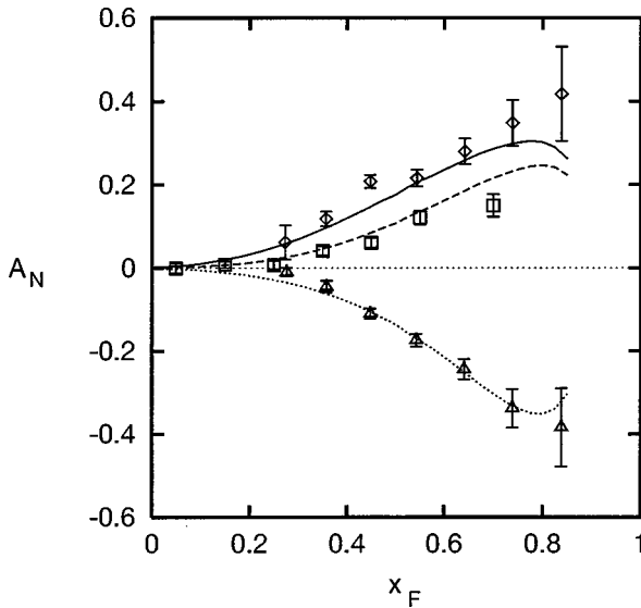
FIG. 2. Single spin asymmetry for pion production, p^\dagger p \rightarrow \pi X . The data points are the E704 experimental single spin asymmetries [3] for \pi^+ (diamonds), \pi^0 (squares), and \pi^- (triangles). The solid line is our best fit for \pi^+ , the dashed line for \pi^0 , and the dotted line for \pi^- , obtained under the assumption of the Collins effect only.
