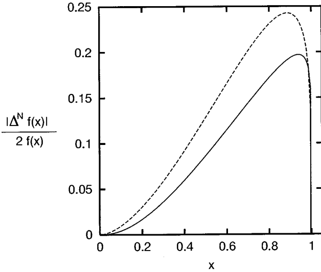
FIG. 4. The ratio between |\Delta^N f_{\text{val}}| and twice the valence unpolarized distribution function f , Eq. (29), as a function of x . The solid line refers to u quarks and the dashed line to d quarks. Notice that in both cases |\Delta^N f|/2f \rightarrow 0 for x \rightarrow 1 .
