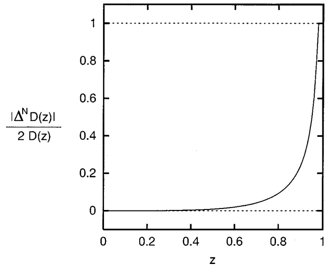
FIG. 3. The ratio between |\Delta^N D_{\text{val}}| and twice the valence unpolarized fragmentation function D , Eq. (28), as a function of z . Notice that |\Delta^N D|/2D = 1 for z \geq 0.97742 .
