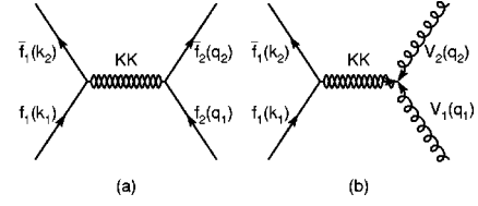
FIG. 1. Feynman diagrams for (a) four-fermion interactions and (b) \bar{f}fVV interactions. We represent KK states by double-sinusoidal curves.
