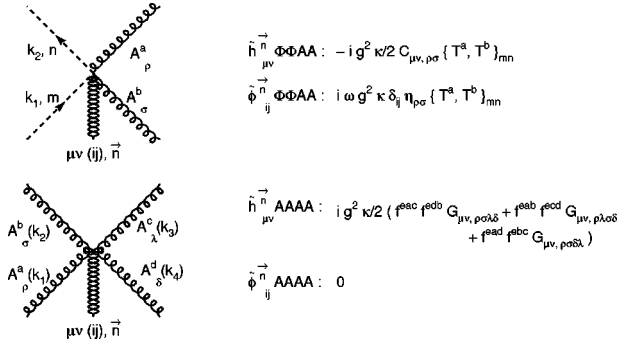
FIG. 6. Five-point vertex Feynman rules. g^2\{T^a, T^b\} \rightarrow 2e^2 Q_f^2 for QED. The symbols C_{\mu\nu,\rho\sigma} and G_{\mu\nu,\rho\sigma\lambda\delta} are defined in Eqs. (A10) and (A14).
