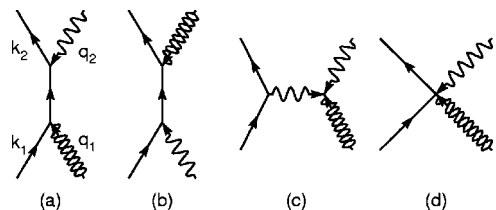
FIG. 2. Feynman diagrams for e^-e^+ \rightarrow \gamma + KK .
