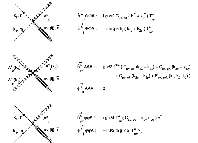
FIG. 5. Four-point vertex Feynman rules. g is the gauge coupling and f^{abc} the structure constant of the Lie algebra; gT^a \rightarrow eQ_f for QED. The symbols C_{\mu\nu,\rho\sigma} and F_{\mu\nu,\rho\sigma\lambda}(k_1, k_2, k_3) are defined in Eqs. (A10) and (A13).
