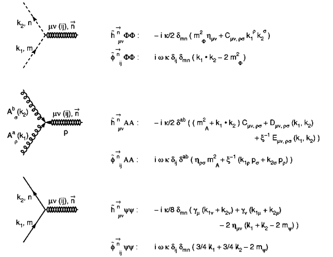
FIG. 4. Three-point vertex Feynman rules. The KK states are plotted in double-sinusoidal curves. The symbols C_{\mu\nu,\rho\sigma} , D_{\mu\nu,\rho\sigma}(k_1, k_2) , and E_{\mu\nu,\rho\sigma}(k_1, k_2) are defined in Eqs. (A10), (A11), and (A12), respectively. m_{\Phi} , m_A , and m_{\psi} are masses of the scalar, vector, and fermion. \omega = \sqrt{2/3}(n+2) , \kappa = \sqrt{16\pi G_N} , and \xi is the gauge-fixing parameter.
