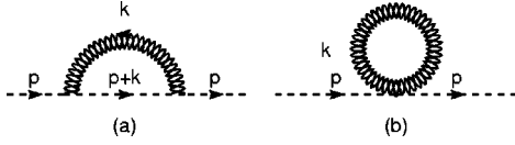
FIG. 3. One-loop self-energy diagrams of the scalar particle.
