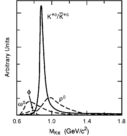
FIG. 9. Simulated relative contributions of the K^{*0}/\bar{K}^{*0} signal (line) and of various resonant backgrounds (dashed lines) to the m_{K\pi} distribution after all analysis cuts.
