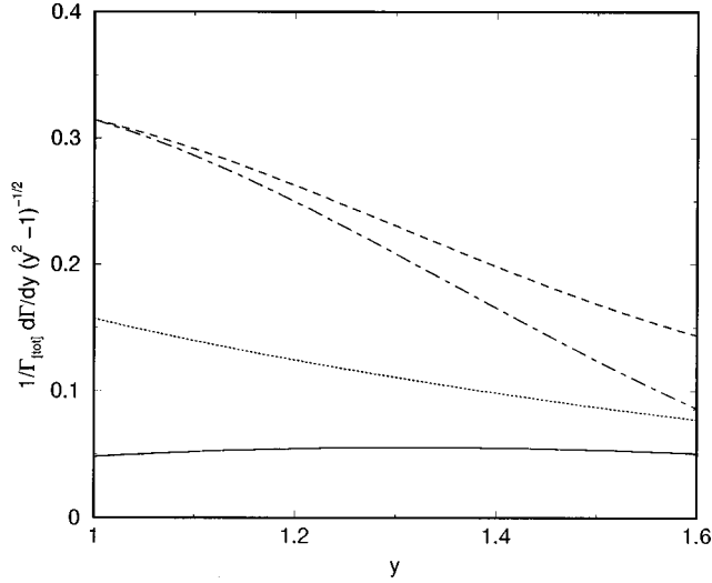
FIG. 3. Decay spectra of the one-particle inclusive decays. Solid line: B \rightarrow D^- l^+ \nu X ; dotted line: B \rightarrow \bar{D}^0 l^+ \nu X ; dashed line: B \rightarrow (D^- + \bar{D}^0) l^+ \nu X , dashed-dotted line: B^0 \rightarrow (D^- + D^{*-}) l^+ \nu .
