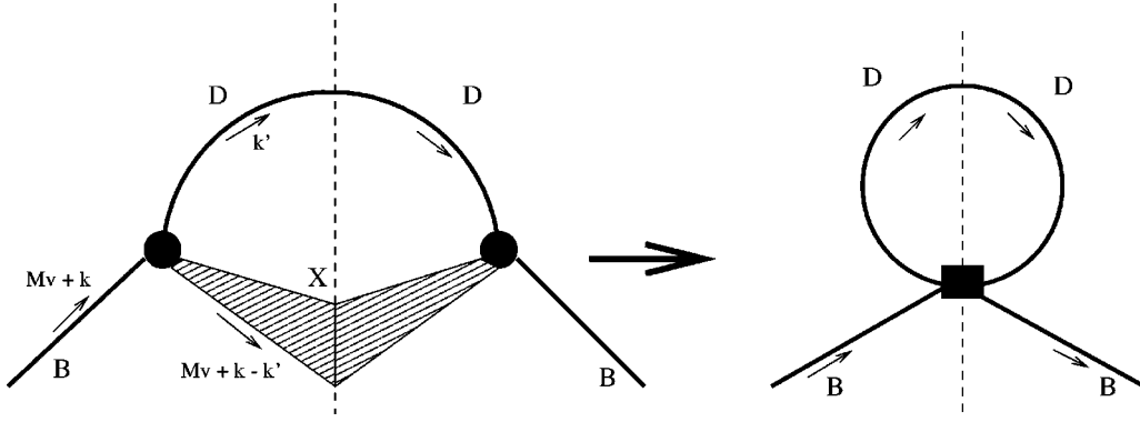
FIG. 1. Illustration of the short distance expansion of Eq. (6).
