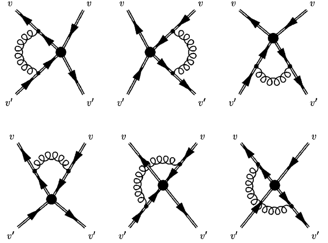
FIG. 2. Feynman diagrams contributing to the one loop anomalous dimensions. The blob represents generically the operators corresponding to the \eta_i and \rho_i .
