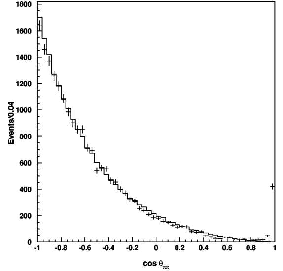
FIG. 1. The distribution of the cosine of the angle between the \pi^+ and \pi^- , \cos \theta_{\pi\pi} , in \psi' \rightarrow \pi^+\pi^-J/\psi , J/\psi \rightarrow e^+e^- events (dots with error bars) compared with the distribution of Monte Carlo data (histogram). The data have background near \cos \theta_{\pi\pi} = 1 .
