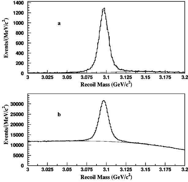
FIG. 2. (a) Number of events versus m_{\pi^+\pi^-}^{recoil} , the mass recoiling against the two \pi 's, for \psi(2S) \rightarrow \pi^+\pi^- J/\psi, J/\psi \rightarrow l^+l^- events. The histogram is data, and the smooth curve is a BWG (“signal”) plus a third order polynomial (“background”). (b) Number of events versus m_{\pi^+\pi^-}^{recoil} for inclusive events. The histogram is data, and the smooth curve is a BWG (signal) with parameters determined from (a) plus a fourth order polynomial (background).
