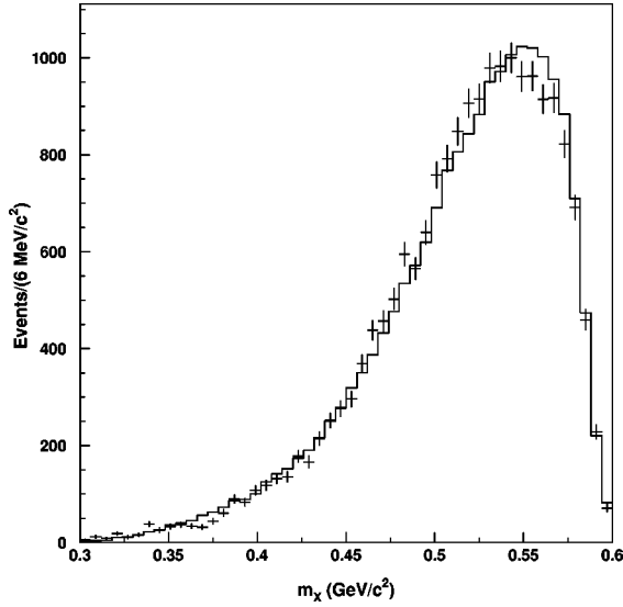
FIG. 3. Number of events versus m_X . The points with error bars are data, and the histogram is Monte Carlo data.
