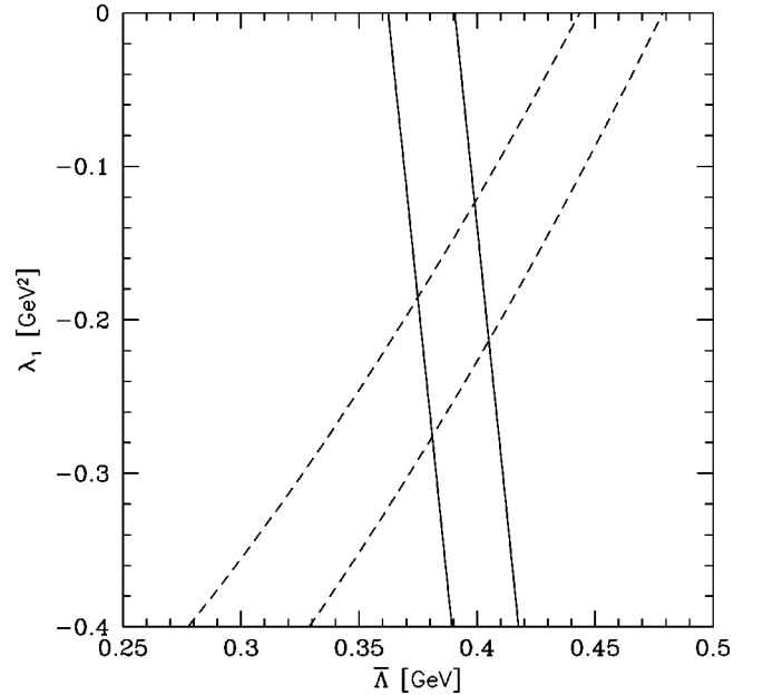
FIG. 6. \langle S_H \rangle (solid bands) and \langle S_H^2 \rangle (dashed bands) correlation in (\lambda_1, \bar{\Lambda}) space for fixed values \langle S_H \rangle = 1.64 GeV 2 and \langle S_H^2 \rangle = 4.48 GeV 4 , corresponding to the central values in Table III. The curves are forced to meet at the point \lambda_1 = -0.2 GeV 2 and \bar{\Lambda} = 0.39 GeV.
