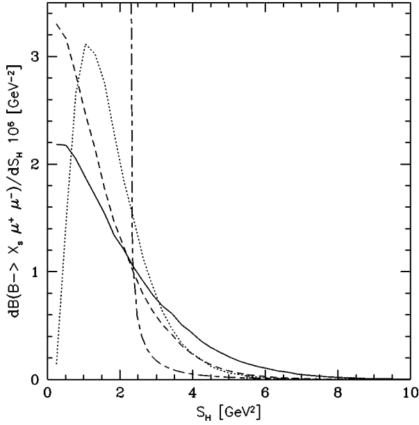
FIG. 9. Hadronic invariant mass spectrum in the Fermi motion model and parton model, based on the perturbative contribution only. The solid, dotted, dashed curve corresponds to the parameters (\lambda_1, \bar{\Lambda}) = (-0.3, 0.5), (-0.1, 0.4), (-0.15, 0.35) in (\text{GeV}^2, \text{GeV}) , respectively. The parton model (long-short dashed) curve is drawn for m_b = 4.85 \text{ GeV} .
