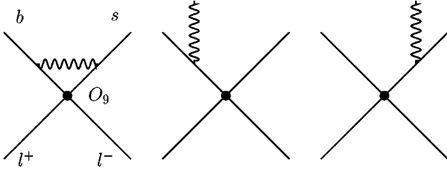
FIG. 1. Feynman diagrams contributing to the explicit order \alpha_s corrections of the operator O_9 . Curly lines denote a gluon. Wave function corrections are not shown.
