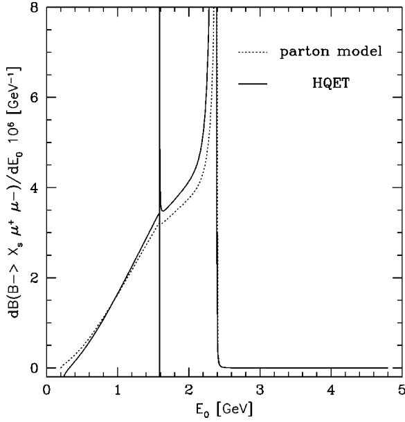
FIG. 5. Hadron energy spectrum d\mathcal{B}(B \rightarrow X_s l^+ l^-)/dE_0 in the parton model (dotted line) and including leading power corrections (solid line). For m_b/2 < E_0 \leq m_b the distributions coincide. The parameters used for this plot are the central values given in Table I and the default values of the HQET parameters specified in text.
