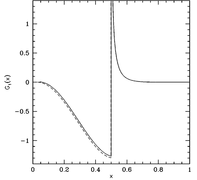
FIG. 2. The function G_1(x) is shown for m_s = 0.2 GeV (solid line) and for the massless case corresponding to Eq. (29) (dashed line).
