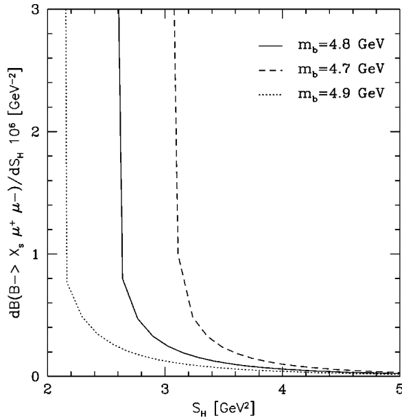
FIG. 4. The differential branching ratio d\mathcal{B}(B \rightarrow X_s l^+ l^-)/dS_H in the hadronic invariant mass, S_H , show for different values of m_b in the range where only bremsstrahlung diagrams contribute. We do not show the result in the full kinematic range as the spectra tend monotonically to zero for larger values of S_H \leq m_B^2 .
