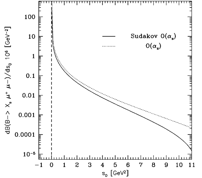
FIG. 3. The differential branching ratio d\mathcal{B}(B \rightarrow X_s l^+ l^-)/ds_0 in the parton model is shown in the \mathcal{O}(\alpha_s) bremsstrahlung region. The dotted (solid) line corresponds to Eq. (30), [Eq. (35)]. The vertical line denotes the one particle pole from b \rightarrow s l^+ l^- . We do not show the full spectra in the range 0 \leq s_0 \leq m_b^2 as they tend to zero for larger values of s_0 .
