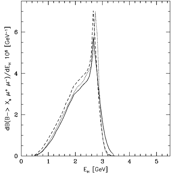
FIG. 7. Hadron energy spectrum in B \rightarrow X_s l^+ l^- in the Fermi motion model based on the perturbative contribution only. The solid, dotted, dashed curve corresponds to the parameters (\lambda_1, \bar{\Lambda}) = (-0.3, 0.5), (-0.1, 0.4), (-0.15, 0.35) in (GeV 2 , GeV), respectively.
