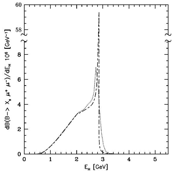
FIG. 8. Hadron energy spectrum in B \rightarrow X_s l^+ l^- based on the perturbative contribution only, in the Fermi motion model (dotted curve) for (p_F, m_q) = (252, 300) (MeV, MeV), yielding m_b^{\text{eff}} = 4.85 GeV, and in the parton model (long-short dashed curve) for m_b = 4.85 GeV.
