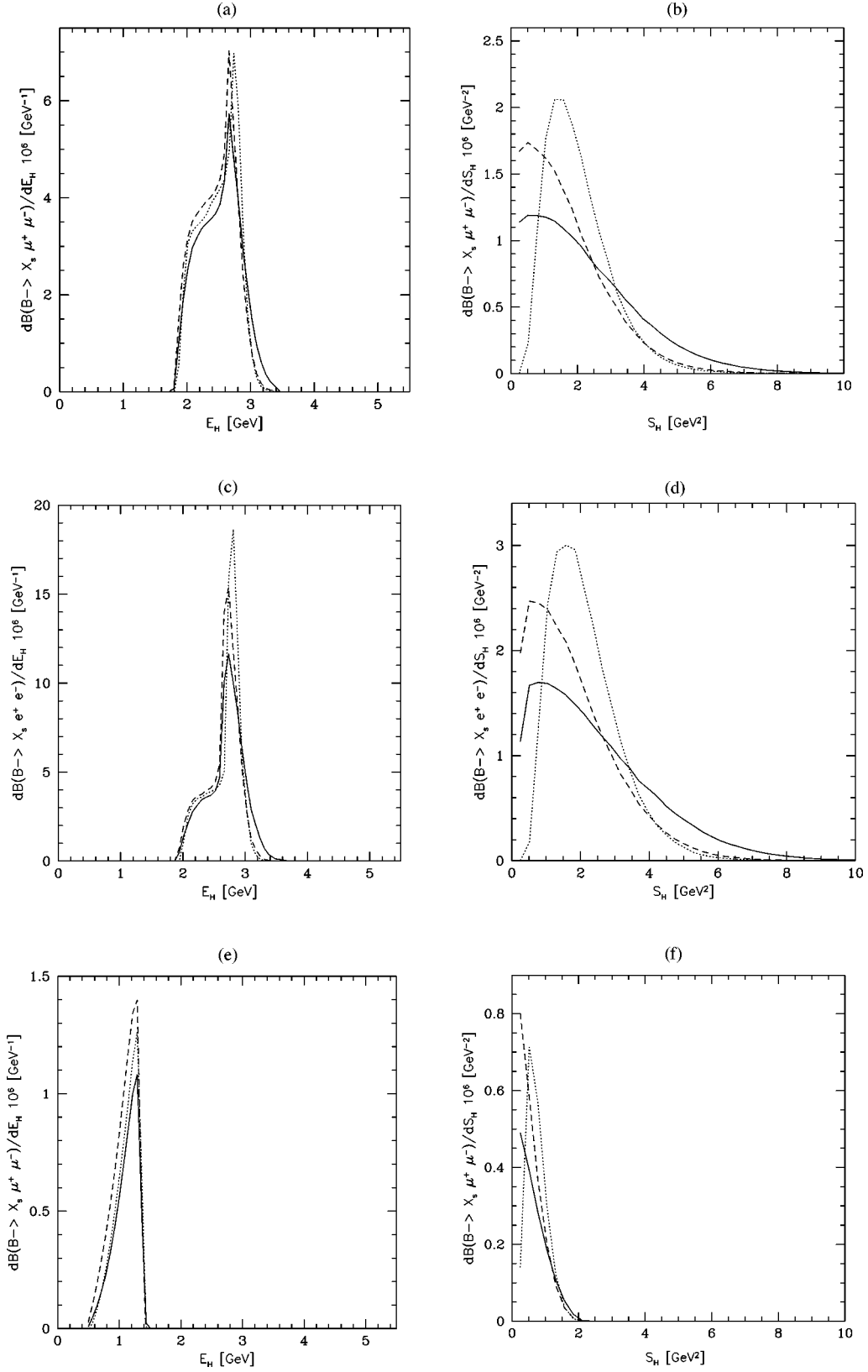
FIG. 10. Hadron spectra in B \rightarrow X_s l^+ l^- in the Fermi motion model with the cuts on the dilepton mass defined in Eq. (78); (a), (c), (e) for the hadronic energy and (b), (d), (f) for the hadronic invariant mass corresponding to cut A, B, C, respectively. The solid, dotted, dashed curves correspond to the parameters (\lambda_1, \bar{\Lambda}) = (-0.3, 0.5), (-0.1, 0.4), (-0.15, 0.35) in (\text{GeV}^2, \text{GeV}) , respectively.
