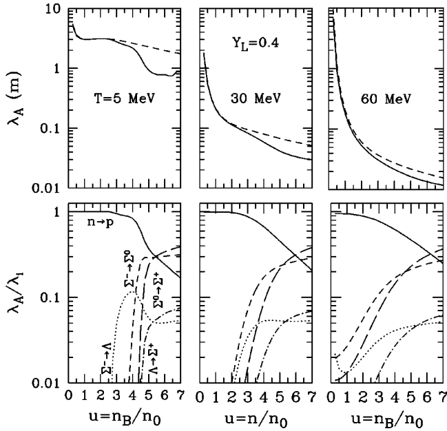
FIG. 19. Absorption mean free paths \lambda = (\sigma/V)^{-1} for neutrino energy E_\nu = \mu_{\nu_e} in matter with fixed lepton number ( Y_L=0.4 ) in the field-theoretical model. Upper panels show both the results for matter without hyperons (dashed curves) and with hyperons (solid curves). Lower panels show the relative contributions to the absorption mean free path for matter with hyperons.
