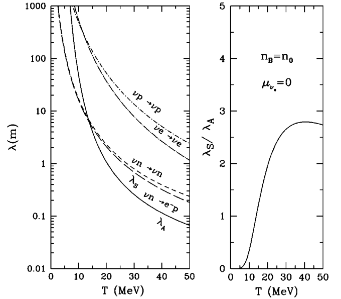
FIG. 7. Temperature dependence of the neutrino mean free path at nuclear saturation density for Y_\nu = 0 and E_\nu = 3T . Left panel: Individual contributions due to scattering and absorption reactions to the mean free path; the long-dashed curve is the total scattering opacity. Right panel: Ratio of the total scattering mean free path to that of absorption.
