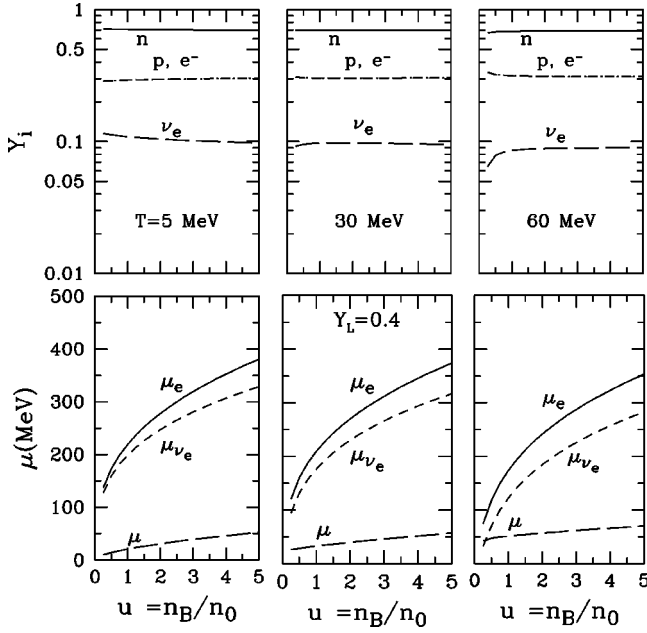
FIG. 2. Composition and chemical potentials for noninteracting matter in beta equilibrium at Y_L=0.4 at different temperatures. Top panels: Individual concentrations Y_i=n_i/n_B , where i=n, p, e^- and \nu_e . Bottom panels: The lepton chemical potentials and \mu = \mu_n - \mu_p = \mu_e - \mu_{\nu_e} .
