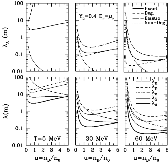
FIG. 9. Neutrino absorption mean free path in neutrino-trapped matter with Y_L=0.4 . Results for the limiting cases discussed in the text are also shown, with the same notation as in Fig. 3.
