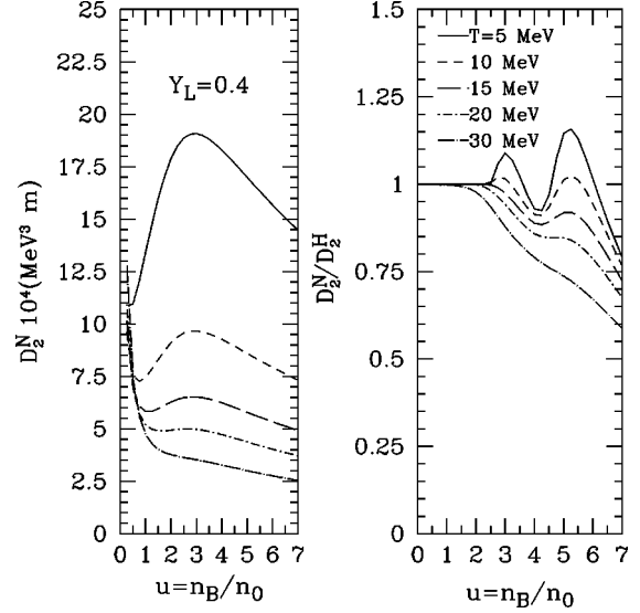
FIG. 24. Neutrino diffusion coefficient D_2 defined in Eq. (91) in matter with and without hyperons for Y_L=0.4 in the field-theoretical model. The left panel shows D_2 as a function of baryon density in matter containing only nucleons and leptons. The ratio of D_2 in matter without hyperons to D_2 in matter with hyperons is shown in the right panel.
