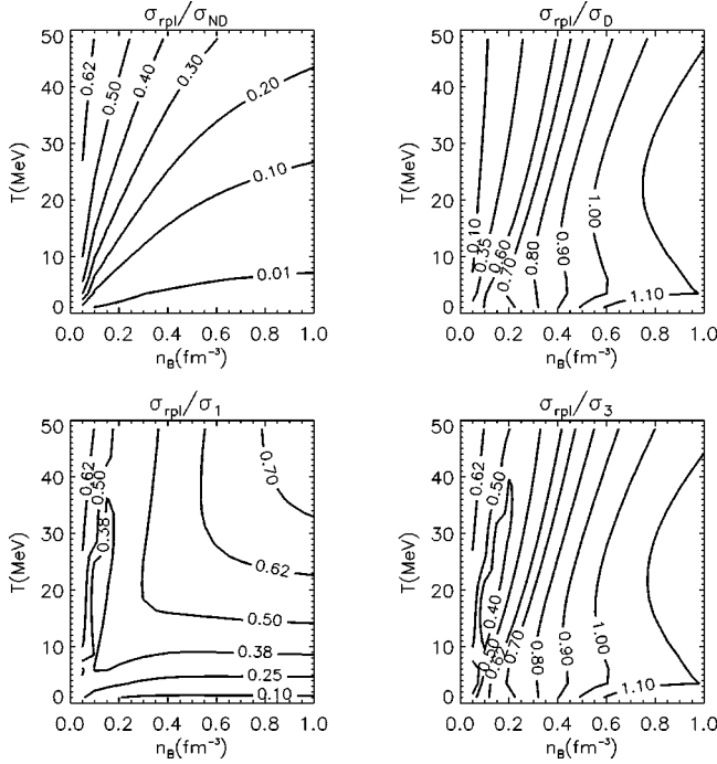
FIG. 17. Comparison with previous cross sections employed in proton-neutron star calculations. The upper panels show comparisons with limiting forms valid for the nondegenerate (left) and degenerate (right) matter. The lower panels show comparisons with interpolated cross sections; the interpolation scheme in Eq. (86) is shown in the left panel and that in Eq. (87) is shown in the right panel.
