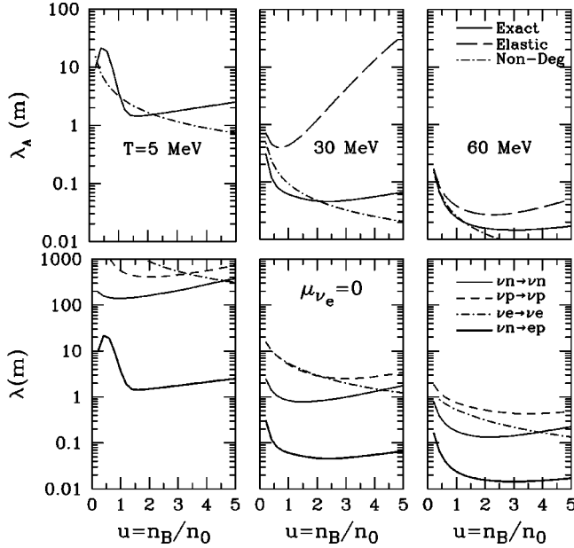
FIG. 12. Upper panel: Neutrino absorption mean free path in neutrino-free matter with the Skyrme model, assuming E_\nu = 3T . The exact and limiting cases discussed in the text are shown, with the same notation as in Fig. 3. For T=5 MeV, the elastic approximation is off-scale. Lower panel: Comparison of absorption and scattering mean free paths for this case.
