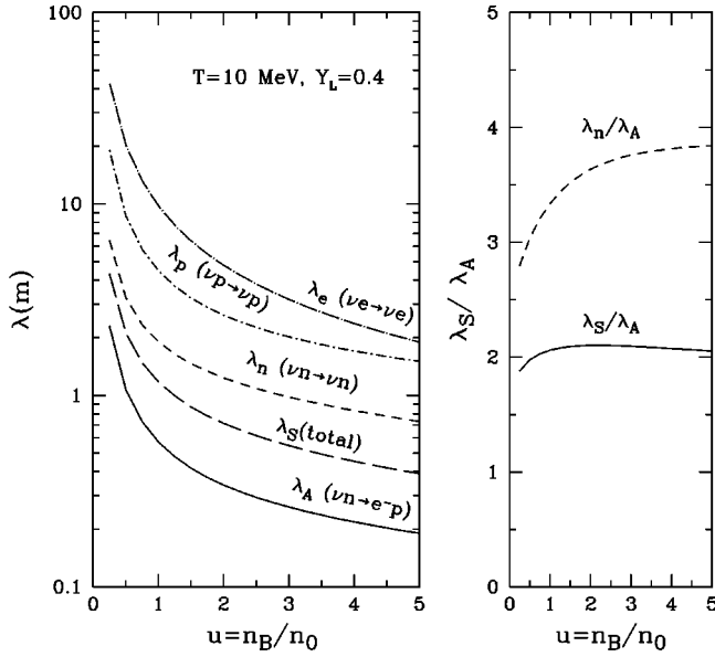
FIG. 4. Comparison between scattering and absorption reactions at T=10 MeV for neutrino-trapped matter ( Y_L=0.4 ), assuming E_\nu=\mu_\nu . The neutrino energy was set equal to the local neutrino chemical potential. In the left panels the contributions to the neutrino mean free path due to individual reactions are shown. In the right panel, the solid curve is the ratio of the scattering to absorption mean free paths and the dashed curve is the neutron scattering/absorption ratio.
