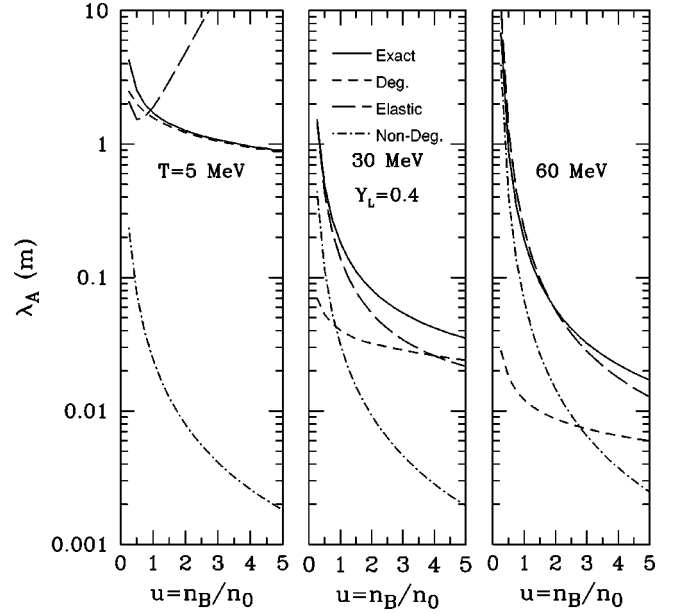
FIG. 3. Absorption mean free paths \lambda = \sigma/V in noninteracting matter in beta equilibrium at different temperatures. The neutrino energy is taken to be the Fermi energy ( E_\nu = \mu_\nu ). The solid curves show exact results from Eqs. (15) and (21), the dashed curves are from the degenerate approximation [Eq. (26)], the dot-dashed curves are the nondegenerate results from Eq. (31), and the long dashed curves represent the elastic approximation from Eq. (34).
