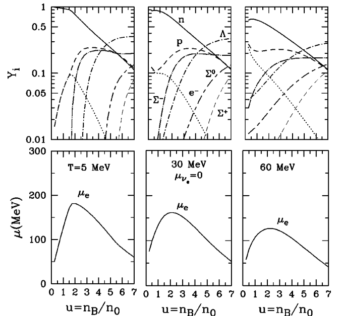
FIG. 21. Compositions (upper panels) and chemical potentials (lower panels) for neutrino-free matter ( Y_\nu=0 ) including hyperons in the field-theoretical model.
