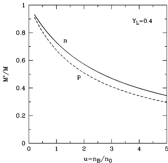
FIG. 10. Neutron (solid curve) and proton (dashed curve) effective masses as a function of baryon density in the Skyrme model. The curves shown are for T=30 MeV.
