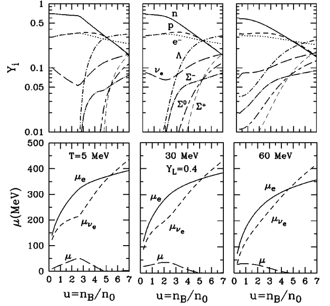
FIG. 18. Compositions (upper panels) and chemical potentials (lower panels) for neutrino-trapped matter ( Y_L=0.4 ) including hyperons in the field-theoretical model. \mu = \mu_n - \mu_p = \mu_e - \mu_{\nu_e} .
