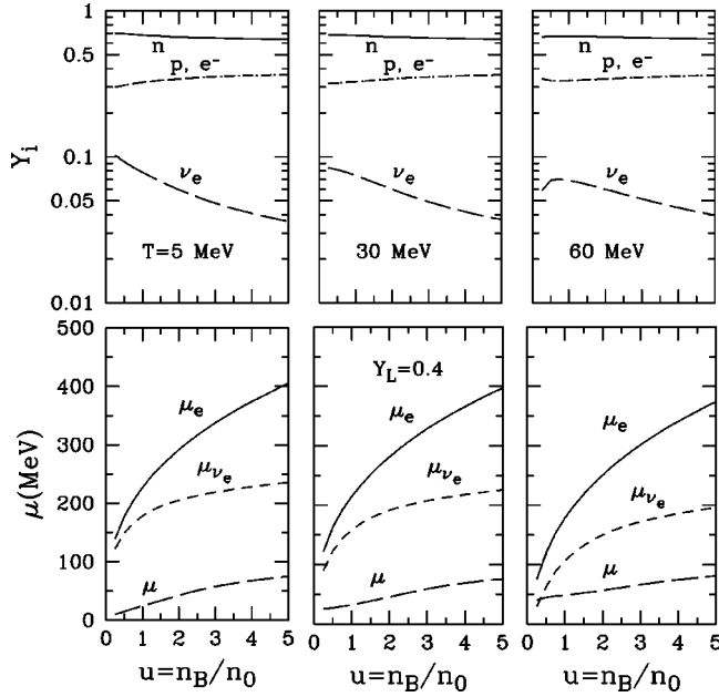
FIG. 13. Compositions (upper panels) and chemical potentials (lower panels) in field-theoretical model for nucleonic matter in beta equilibrium with fixed lepton number Y_L=0.4 .
