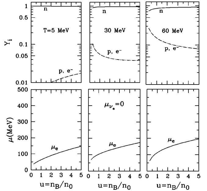
FIG. 5. Compositions and chemical potentials for noninteracting matter in beta equilibrium with no trapped neutrinos ( Y_\nu=0 ) at different temperatures. Top panels: Individual concentrations Y_i=n_i/n_B , where i=n, p , and e^- . Bottom panels: The electron chemical potential \mu_e=\mu_n-\mu_p .
