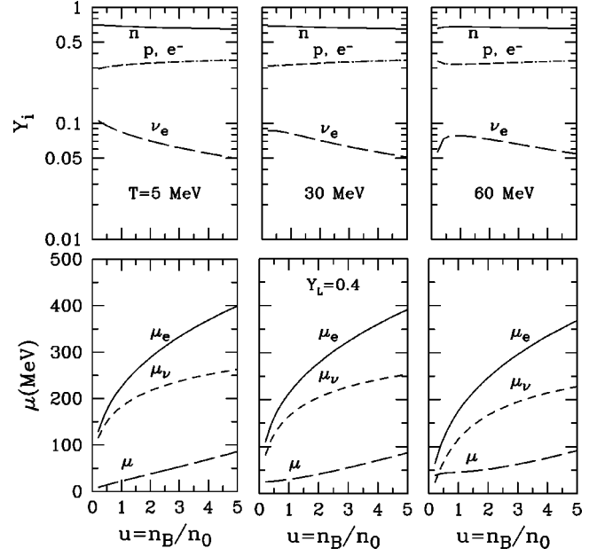
FIG. 8. Particle fractions (upper panels) and lepton chemical potentials (lower panels) in the nonrelativistic potential Skyrme model for Y_L=0.4 at various temperatures. Note that the proton fraction is larger than in the noninteracting case.
