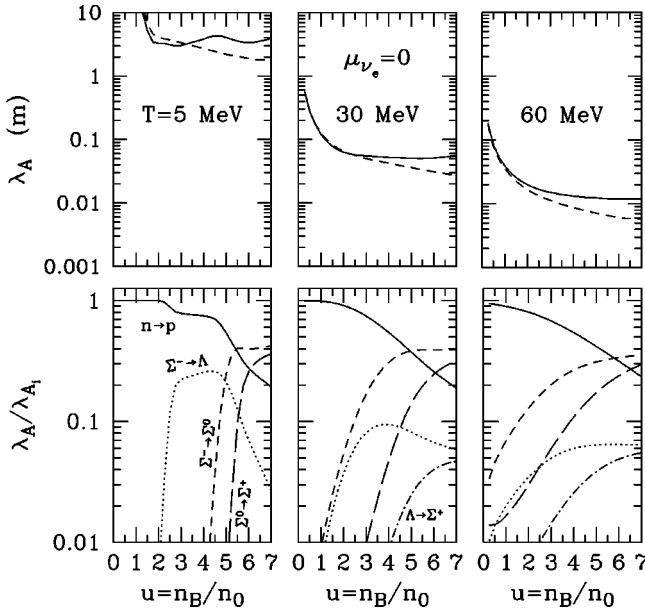
FIG. 22. Absorption mean free paths \lambda = (\sigma/V)^{-1} for neutrino energy E_\nu = 3T in matter with no trapped neutrinos ( Y_\nu = 0 ) in the field-theoretical model. Upper panels show both the results for matter without hyperons (dashed curves) and with hyperons (solid curves). Lower panels show the relative contributions to the absorption mean free path for matter with hyperons.
