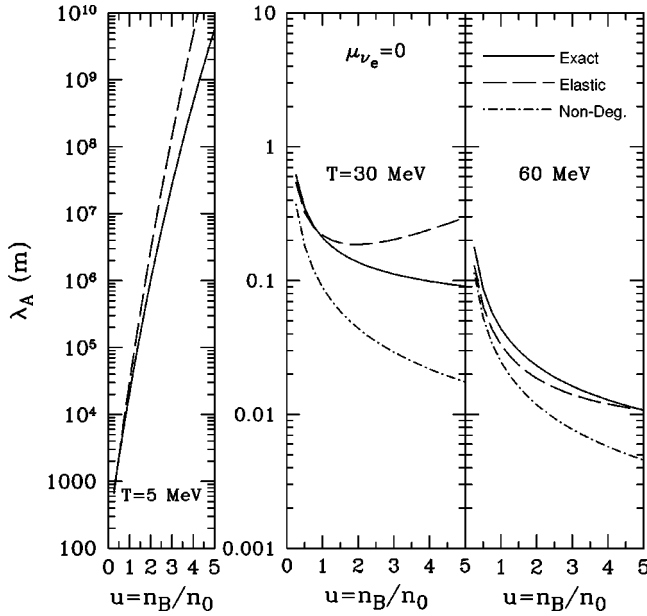
FIG. 6. Absorption mean free paths \lambda = \sigma/V in noninteracting matter in beta equilibrium with no trapped neutrinos at different temperatures. The neutrino energy is taken to be E_1 = 3T . The left-most panel clearly shows that at low temperatures the mean free path is very large since the reaction is kinematically suppressed.
