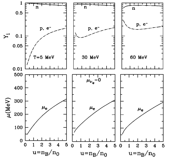
FIG. 11. Compositions (upper panels) and electron chemical potentials (lower panels) for neutrino-free matter at various temperatures in the Skyrme model. Note that the proton fraction is larger when compared with the noninteracting case and, at low densities, is quite sensitive to the temperature.
