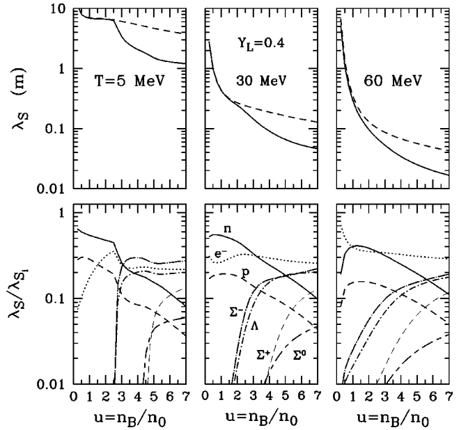
FIG. 20. Scattering mean free paths for neutrino energy E_\nu = \mu_{\nu_e} in matter with fixed lepton number ( Y_L=0.4 ) in the field-theoretical model. Upper panels show the results for the total scattering mean free path for matter without hyperons (dashed curves) and with hyperons (solid curves). Lower panels show the relative contributions to the scattering mean free path for matter with hyperons.
