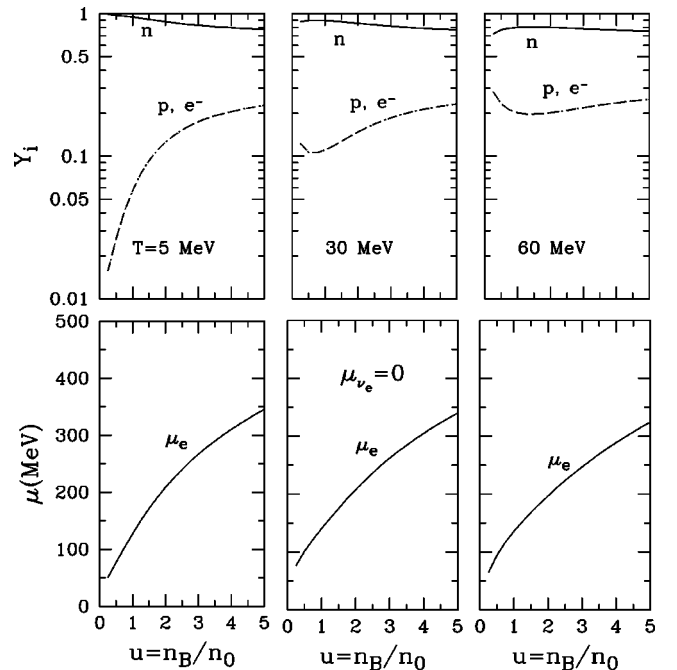
FIG. 15. Composition (upper panels) and chemical potentials (lower panels) matter in beta equilibrium with no trapped neutrinos ( Y_\nu=0 ) for the field-theoretical model.
