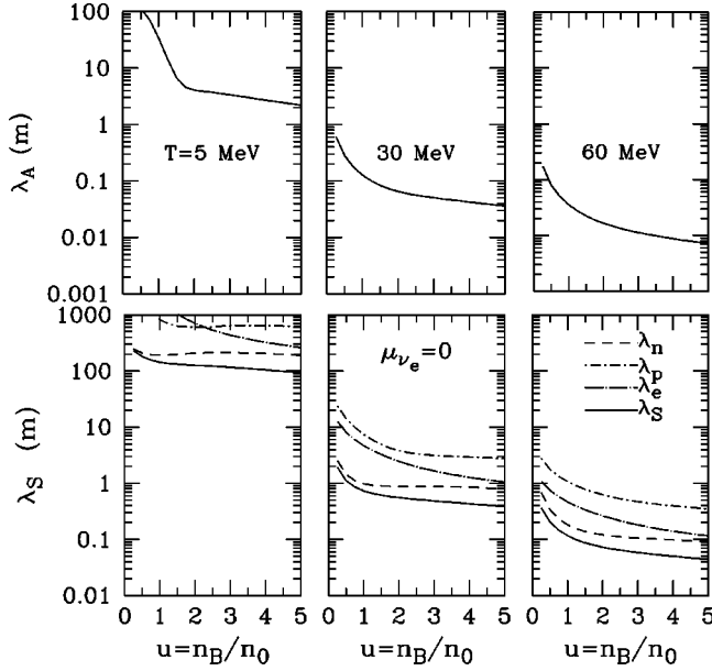
FIG. 16. Absorption (upper panels) and scattering (lower panels) mean free paths \lambda = \sigma/V for neutrino energy E_\nu = 3T in matter with no trapped neutrinos for the field-theoretical model.
