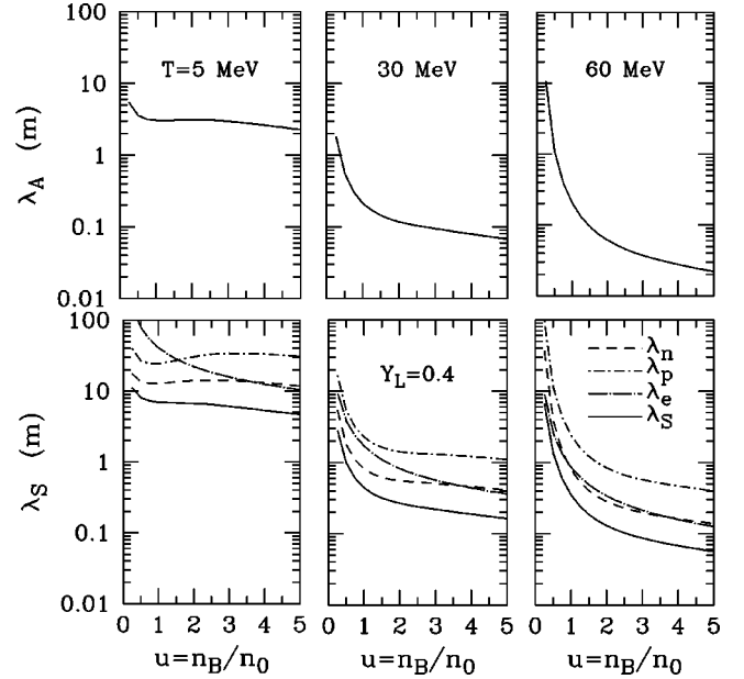
FIG. 14. Absorption (upper panels) and scattering (lower panels) mean free paths \lambda = \sigma/V for neutrino energy E_\nu = \mu_{\nu_e} in beta equilibrium matter with Y_L=0.4 , for the field-theoretical model.
