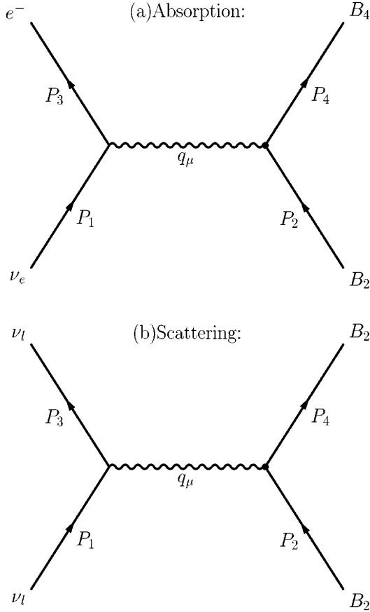
FIG. 1. Lowest order Feynman diagram for \nu_l + B_2 \rightarrow l + B_4 . The symbols B_i and l denote baryons and leptons, respectively. P_i are the particles' four-momenta and q_\mu = (q_0, \vec{q}) is the four-momentum transfer. Figure (a) is the absorption reaction and Fig. (b) is the scattering reaction.
