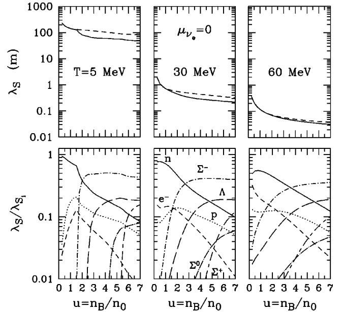
FIG. 23. Scattering mean free path for neutrino energy E_\nu = 3T in matter with no trapped neutrinos ( Y_\nu = 0 ) in the field-theoretical model. Upper panels show the results for the total scattering mean free path for matter without hyperons (dashed curves) and with hyperons (solid curves). Lower panels show the relative contributions to the scattering mean free path for matter with hyperons.
