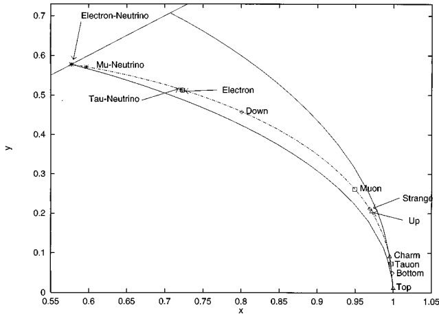
FIG. 3. The locations of the various fermion states on the common trajectory.
