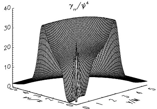
FIG. 1. We show the radial metric function \gamma_{rr}/\psi^4 for the evolution of the distorted black hole data set (a,b,w,n,c) = (0.5,0,1,2,0) at time t=27.2M . The evolution was performed with 150^3 grid points, although data from only the inner 100^3 grid points are shown to bring out detail. The resolution was \Delta x=0.0544M .
