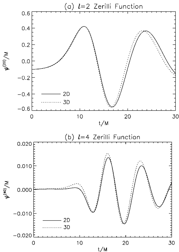
FIG. 2. We show the (a) \ell=2 and (b) \ell=4 Zerilli functions vs time, extracted during 2D and 3D evolutions of the data set (a,b,w,n,c)=(0.5,0,1,2,0) . The functions were extracted at a radius of 8.7M . The 2D data were obtained with 202 \times 54 grid points, giving a resolution of \Delta\eta = \Delta\theta = 0.03 . The 3D data were obtained using 300^3 grid points and a resolution of \Delta x = 0.0816M .
