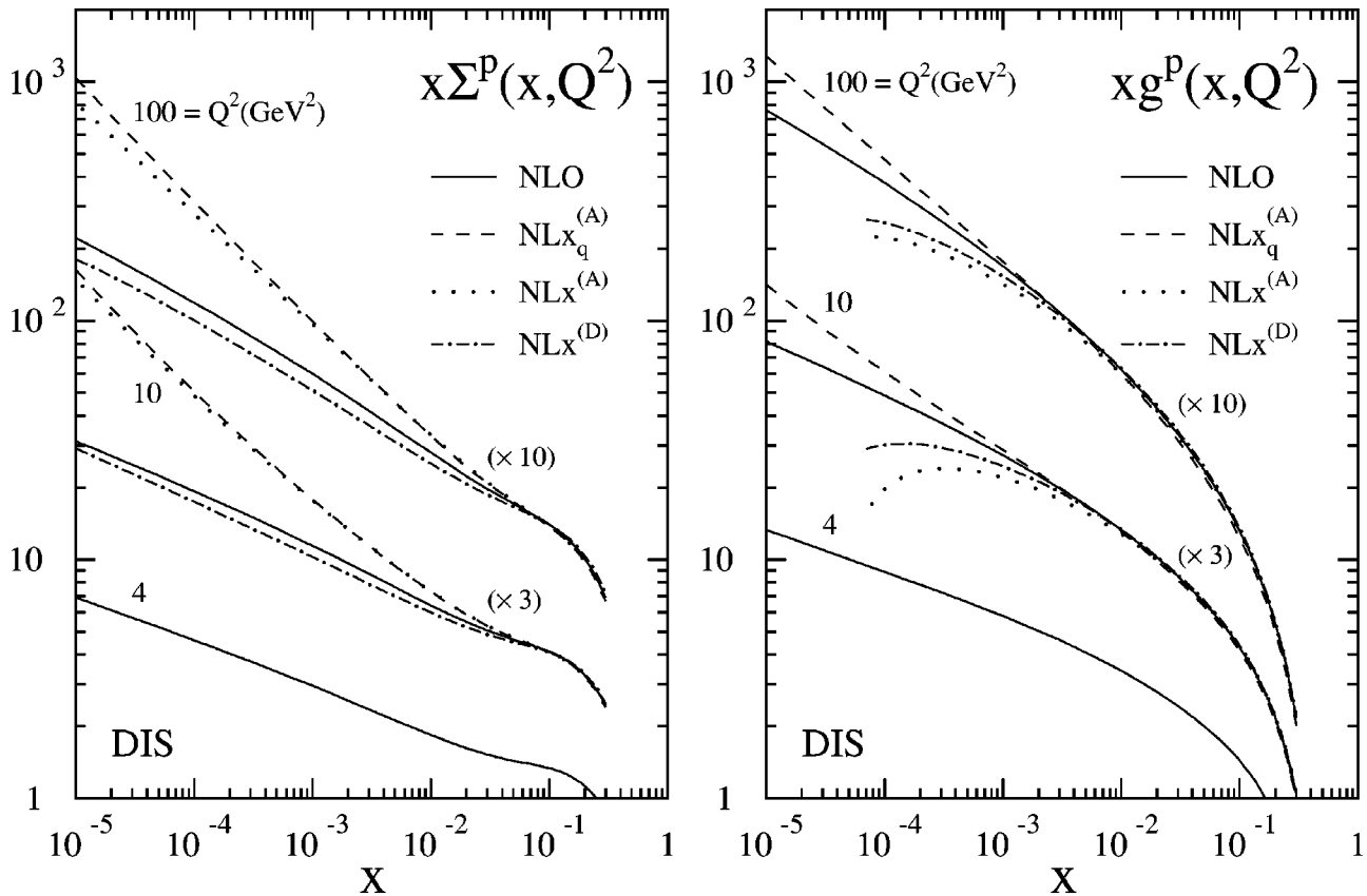
FIG. 1. The small- x evolution of the singlet quark and gluon densities including the resummed \text{NLx}_q kernels [2] and the new terms of the gluon-gluon anomalous dimension [9,12] as compared to the NLO results. Two prescriptions for implementing the momentum sum rule have been applied.
