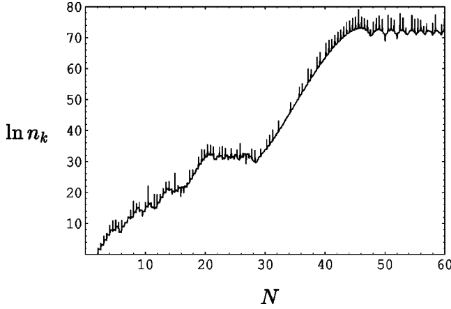
FIG. 3. The exponential growth of the occupation number n_k of \chi -particles, for k = \bar{m}_\phi , as a function of the number of oscillations of the field \phi , N = \bar{m}_\phi t / 2\pi . One can distinguish here the broad stochastic resonance regime. The typical value of the growth parameter is \mu \approx 0.13 during the last stages of preheating.
