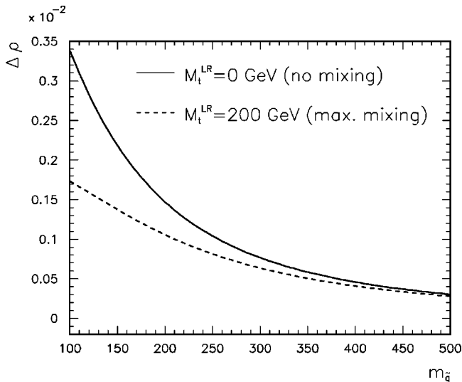
FIG. 2. One-loop contribution of the (\tilde{t}, \tilde{b}) doublet to \Delta\rho as a function of the common squark mass m_{\tilde{q}} for \theta_{\tilde{t}} = 0 and \theta_{\tilde{t}} \sim -\pi/4 (with \tan\beta = 1.6 , M_b^{LR} = 0 , and M_t^{LR} = 0 or 200 GeV).
