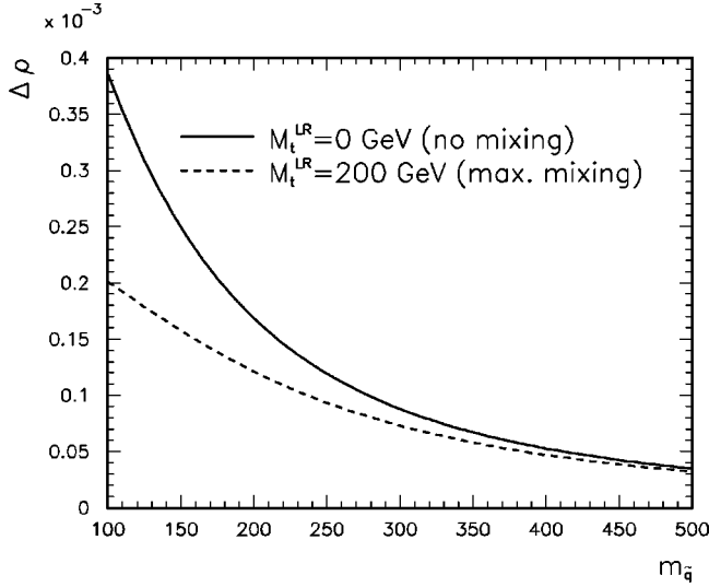
FIG. 7. \Delta\rho_{1,\text{gluon}}^{\text{SUSY}} as a function of m_{\tilde{q}} for the scenarios of Fig. 2.
