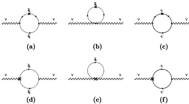
FIG. 5. Counterterm contributions to the gauge-boson self-energies at two-loop order.
