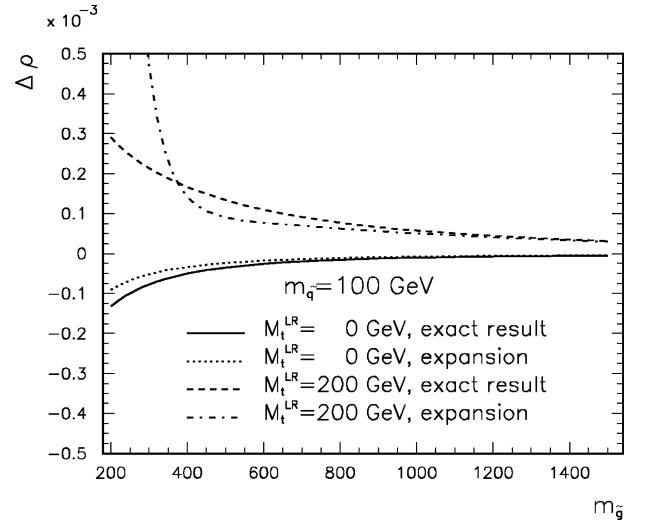
FIG. 10. Comparison between the exact result for \Delta\rho_{1,\text{gluino}}^{\text{SUSY}} and the result of the expansion, Eq. (24), up to \mathcal{O}(1/m_{\tilde{g}}^3) for the two scenarios of Fig. 2; m_{\tilde{q}}=100 GeV.
