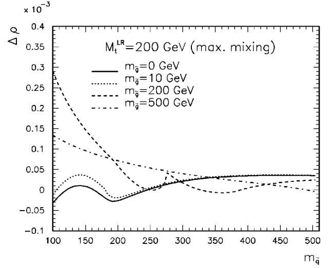
FIG. 9. \Delta\rho_{1,\text{gluino}}^{\text{SUSY}} as a function of m_{\tilde{q}} in the maximal mixing scenario; \tan\beta=1.6 and m_{\tilde{g}}=0, 10, 200, and 500 GeV.
