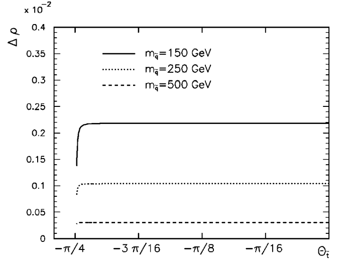
FIG. 3. Dependence of the one-loop contribution \Delta\rho_0^{\text{SUSY}} on the top-squark mixing angle \theta_{\tilde{t}} . The parameters are the same as in Fig. 2.
