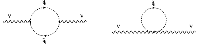
FIG. 1. Feynman diagrams for the contribution of scalar quark loops to the gauge boson self-energies at one-loop order.
