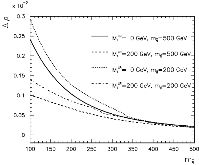
FIG. 11. \Delta\rho_0^{\text{SUSY}} calculated with one-loop corrected squark masses as a function of m_{\tilde{q}} for \theta_{\tilde{t}}=0 and \theta_{\tilde{t}} \sim -\pi/4 ( \tan\beta=1.6 , M_t^{LR}=0 or 200 GeV) and two values of m_{\tilde{g}} .
