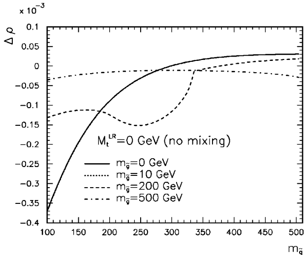
FIG. 8. \Delta\rho_{1,\text{gluino}}^{\text{SUSY}} as a function of m_{\tilde{q}} in the no-mixing scenario; \tan\beta=1.6 and m_{\tilde{g}}=0, 10 (the plots are indistinguishable), 200, and 500 GeV.
