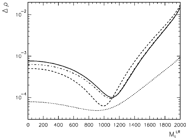
FIG. 12. \Delta\rho_0^{\text{SUSY}} as a function of M_t^{LR} for \tan\beta=1.6 and for M_{\tilde{t}_L}/M_{\tilde{t}_R}=1000/300 (dotted line; the lines for tree-level and one-loop parameters are not distinguishable) and 300/1000 (solid line for tree-level parameters; for the one-loop parameters, dash-dotted line for m_{\tilde{g}}=200 GeV and dashed line for m_{\tilde{g}}=500 GeV).
