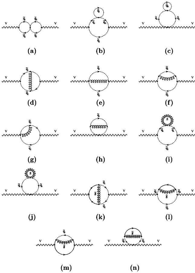
FIG. 4. Feynman diagrams for the contribution of scalar quark loops to the gauge-boson self-energies at two-loop order.
