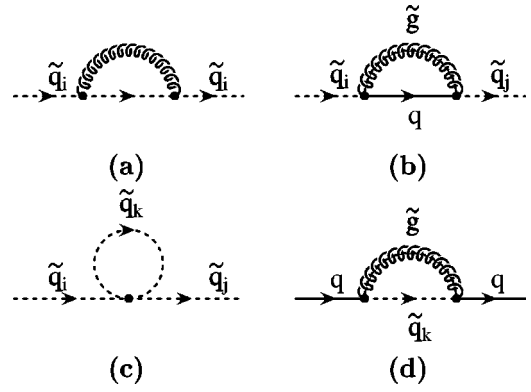
FIG. 6. One-loop diagrams contributing to the squark mass and mixing angle counterterms.
