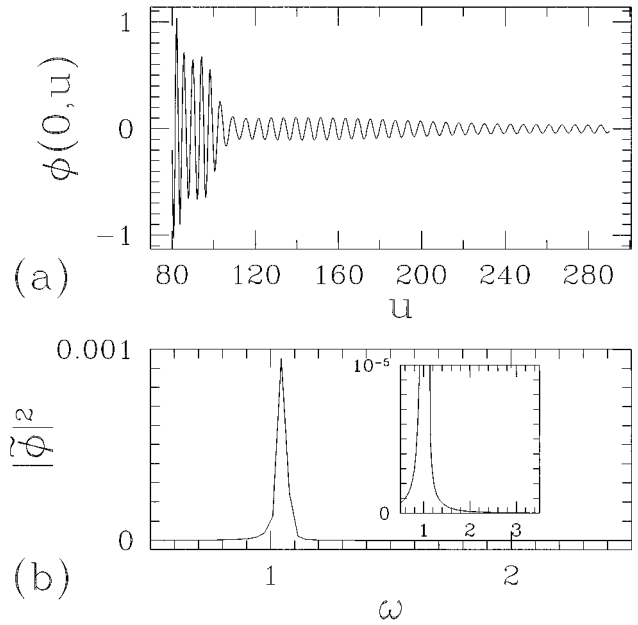
FIG. 2. (a) The time evolution of \phi as a function of retarded time u at the origin for the same evolution as in Fig. 1, but after the nearly critical phase which ends at u \approx 100 . The solution is essentially periodic, with a low-frequency amplitude modulation. (b) The squared amplitude of the discrete Fourier transform of the field for u \geq 100 . The fundamental oscillation has an angular frequency \omega_0 \sim 1.05\mu , which suggests that it is determined by the scalar field mass (which is set to unity). The inset demonstrates that other harmonics are not strongly excited in this solution. For other initial data sets, we find that the amplitude of the oscillations tends to decay slowly, and the solutions are dispersing.
