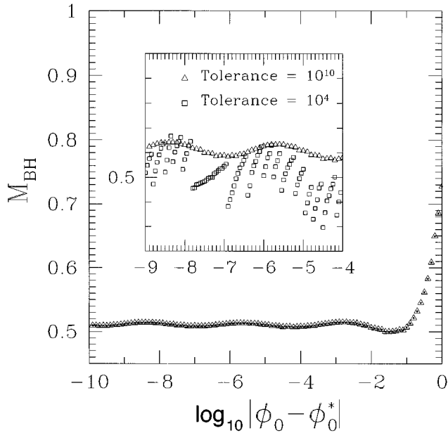
FIG. 3. The black-hole mass M_{\text{BH}} as a function of \log_{10}|\phi_0 - \phi_0^*| for supercritical evolutions with \mu = 1.0 . The results displayed are for the initial data set (iii) in Table I with r_0 = 2.0 and \sigma = 10.0 . The critical point was determined to be \phi_0^* = 3.872\,452\,334\,59 with an initial radial discretization \Delta r = 0.05 . The black hole tolerance parameter (see text) was set at 10^{10} . The inset shows results obtained from the same evolution, but with a lower black hole tolerance level of 10^4 . For low values of the tolerance the mass spectrum exhibits spurious discontinuities.
