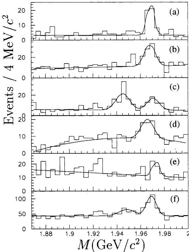
FIG. 1. Mass distribution of D_s single tags. (a) \phi\pi^+ , (b) \bar{K}^{*0}K^+ , (c) K_S^0 K^+ , (d) K_S^0 K^- \pi^+ \pi^+ , (e) f_0\pi^+ , and (f) combined.
