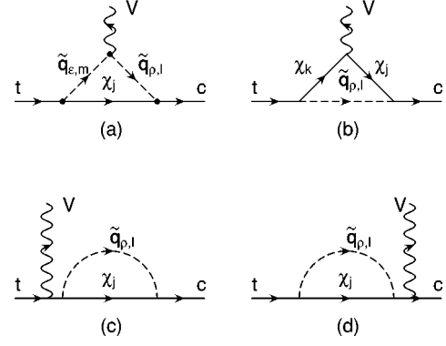
FIG. 1. Feynman diagrams for one-loop electroweaklike supersymmetric contributions to the t - c - V ( V = \gamma, Z, g ) vertex. Here \chi represents the chargino or the neutralino and \tilde{q} represents the down-type or up-type squarks, respectively. The subscripts are explained in the text. The arrows on the squark lines indicate the direction of flow of flavor; the arrows on the gauge bosons indicate the direction of momentum flow. Diagram (b) is absent for V = g , and for V = \gamma when \chi = \chi^0 .
