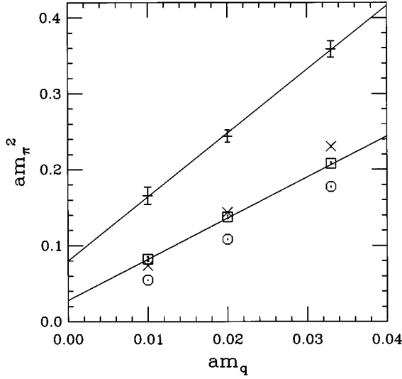
FIG. 1. The squared pion masses versus quark mass for the Wilson gauge action at 6/g^2=5.85 . The plusses and crosses are the \pi_2 and Goldstone \pi masses with the conventional fermion action, and the squares and octagons are the \pi_2 and Goldstone \pi masses with a staple weight w=0.4 . The lines are linear fits to the squared non-Goldstone pion masses.
