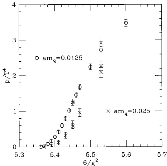
FIG. 6. The pressure obtained from integrating \langle \square \rangle with respect to 6/g^2 at constant am_q . The values from the quark mass integrations (fancy squares) are also shown for comparison.
