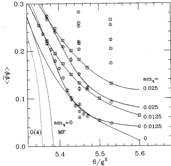
FIG. 4. \langle \bar{\psi}\psi \rangle as a function of 6/g^2 and am_q . The difference in the hot (octagons) and cold (squares) values is related to the interaction measure. \langle \bar{\psi}\psi \rangle on the hot lattices also serves as an order parameter for the system. Lines depict fits to O(4) and mean field singular forms of the free energy plus analytic terms to \langle \square \rangle , \langle \bar{\psi}\psi \rangle , and their derivatives [Eqs. (5)–(8)]. Only points with am_q \leq 0.025 were included in the fits. The difference between O(4) (dotted line) and mean field forms (dashed line) is not discernible at the quark masses where simulations were run. Extrapolations to m_q=0 , however, give different critical couplings. Solid lines correspond to polynomial fits to the cold data and the corresponding extrapolation to am_q=0 .
