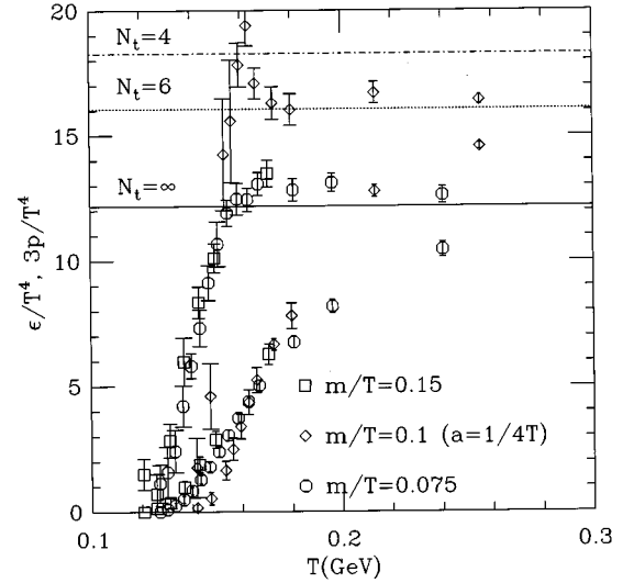
FIG. 9. The equation of state along lines of constant m_q/T . The octagons denote am_q=0.0125 results, squares am_q=0.025 . The diamonds indicate an earlier result on N_t=4 lattices. Horizontal lines correspond to Stefan-Boltzmann laws for N_t=4, 6 , and the continuum. The energy density increases rapidly near the crossover while the pressure (lower curve for each symbol) rises smoothly.
