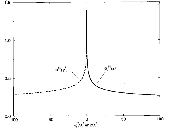
FIG. 1. Plot of the spacelike and timelike definitions of the one-loop running coupling constants, \bar{a}^{(1)}(q^2) and \bar{a}_s^{(1)}(s) . The abscissa is, respectively, -q^2/\Lambda^2 and s/\Lambda^2 for the two functions. Here, we have displayed \alpha = 4\pi a and have used N_f = 3 in \beta_0 .
