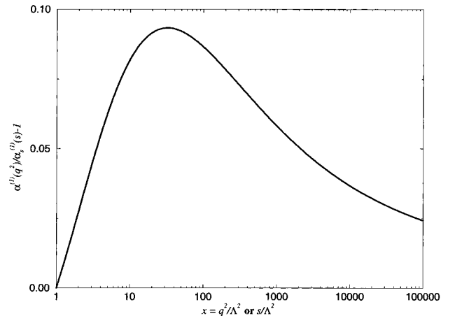
FIG. 2. Plot of the relative difference of the two coupling constants shown in Fig. 1, \bar{a}^{(1)}(x)/\bar{a}_s^{(1)}(x) - 1 . Here, the argument is x = q^2/\Lambda^2 for \bar{a} and x = s/\Lambda^2 for \bar{a}_s .
