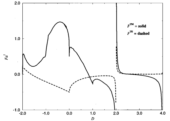
FIG. 1. A plot of the TM Casimir stress F_c^{\text{TM}} for -2 < D < 4 on a spherical shell, compared with F_c^{\text{TE}} , taken from [8]. For D < 2 ( D < 0 ) the stress F_c^{\text{TM}} ( F_c^{\text{TE}} ) is complex and we have plotted \text{Re}F .
