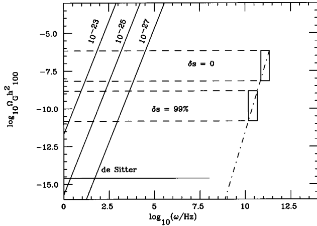
FIG. 1. The area within the dashed lines defines the allowed region for the maximal value of the spectral energy density, for the two cases \delta s=0 and \delta s=0.99 (the plot is done using n_r=10^3 ). The two boxes on the right border define the position of the end point of the spectrum if the end of the string era occurs in the strong coupling regime. For comparison, the flat graviton spectrum of the de Sitter inflationary scenario is plotted for an inflation scale high enough to account for the observed large scale anisotropy. Also plotted are three lines of constant spectral amplitude S_h^{1/2}=10^{-23} , 10^{-25} , and 10^{-27} \text{ Hz}^{-1/2} , as well as the (dash-dotted) “one-graviton” line, along which the end point is shifted as a function of late entropy production.
