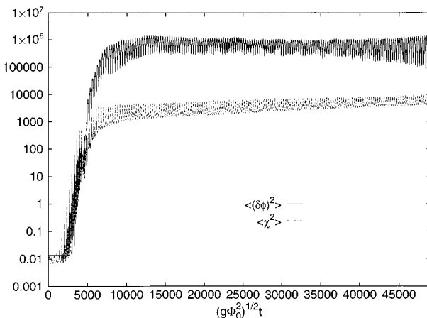
FIG. 2. The variances of the fields as a function of time ( m = 10^{-6}\Phi_0 , \lambda_\chi = \lambda_\phi = 0 , g = 10^{-8} , and \Phi_0 = 10^4 sets the scale for the y axis).
