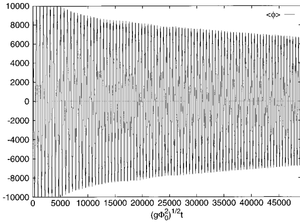
FIG. 1. The EV of the inflaton as a function of time ( m = 10^{-6}\Phi_0 , \lambda_\chi = \lambda_\phi = 0 , g = 10^{-8} , and \Phi_0 = 10^4 sets the scale for the y axis).
