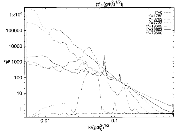
FIG. 6. \chi -field occupation numbers at various times for a model with moderate self-coupling \lambda_{\chi} = 10^{-2} ( m = 10^{-6} \Phi_0 , \lambda_{\phi} = 0 , g = 10^{-8} ).
