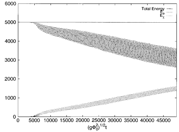
FIG. 3. The energies of the fields as a function of time ( m = 10^{-6}\Phi_0 , \lambda_\chi = \lambda_\phi = 0 , g = 10^{-8} , and \Phi_0 = 10^4 sets the scale for the y axis).
