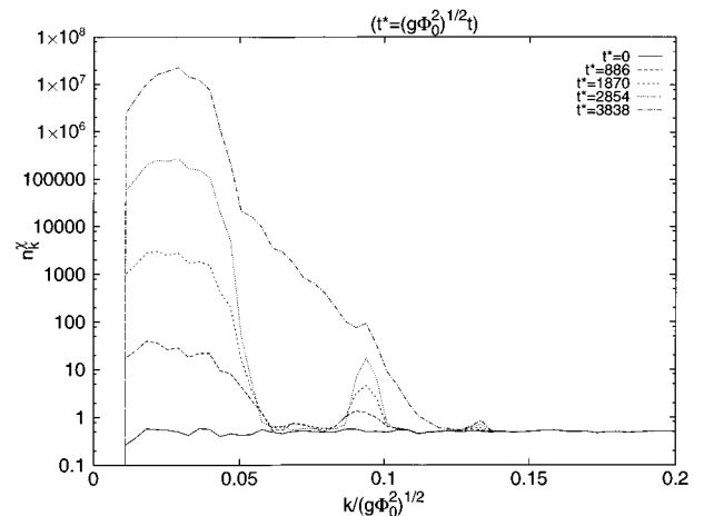
FIG. 4. \chi -field occupation numbers vs momentum at early times. Three resonances are visible.
