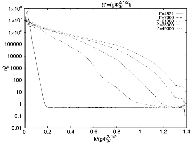
FIG. 5. \chi -field occupation numbers vs momentum at later times, when scatterings dominate.
