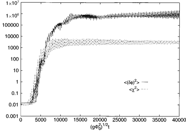
FIG. 7. The variances of the fields as a function of time for a quartic inflaton potential ( m=0 , \lambda_\phi=10^{-12} , g=10^{-8} , and \Phi_0=10^4 sets the scale for the y axis).
