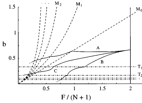
FIG. 1. The scenarios (A), (B), and (C) for the behavior of the coefficient b that determines the superconformal R_{\text{SC}} charges as a function of F/(N+1) , for large, fixed N . The curves meet at F=2(N+1) , where the position and slope can be calculated in perturbation theory. For F near zero it presumably does not make sense to plot b as a continuous function. The lines labeled M_0, M_1, \dots and T_1, T_2, \dots indicate the region where the corresponding operators have scaling dimensions of a free field.
