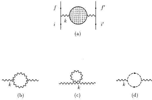
FIG. 1. (a) The gluon self-energy diagrams for the quark-quark scattering. (b) The gluon self-energy diagram with three-gluon interactions. (c) The tadpole diagram for the gluon self-energy. (d) The ghost diagram for the gluon self-energy.
