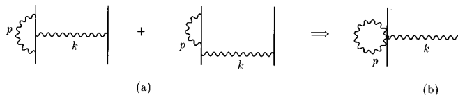
FIG. 2. (a) The vertex diagrams of the first kind for the quark-quark scattering. (b) Their pinch contribution.
