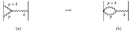
FIG. 3. (a) The vertex diagram of the second kind for the quark-quark scattering. (b) Its pinch contribution.
