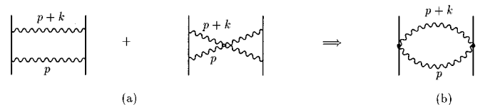
FIG. 4. (a) The box diagrams for the quark-quark scattering. (b) Their pinch contribution.
