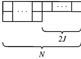
FIG. 1. The Young tableaux for the SU(N_F) flavor representation of the spin- J baryon multiplet.
