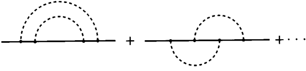
FIG. 4. Two-loop contributions to the baryon mass.
