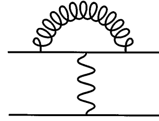
FIG. 5. Example of a quark graph giving rise to the two-body operators \{Q\}\{Q\} and \{Q\sigma^j\}\{Q\sigma^j\} in the effective Lagrangian. The wavy line represents a photon and the curly line represents a gluon. Note that there is a factor of N from the color sum, and so this graph is order 1 in the large- N limit.
