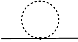
FIG. 2. A contribution to the baryon mass. The solid lines are baryons and the dashed lines are mesons.
