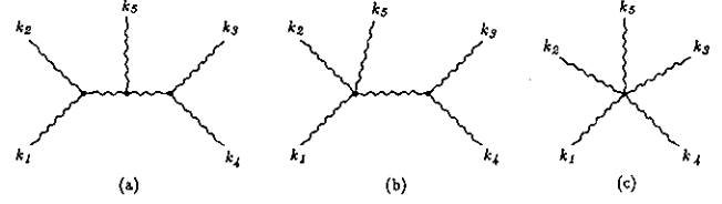
FIG. 2. Higher-order tree amplitude containing nonlinear couplings of gauge particles.
