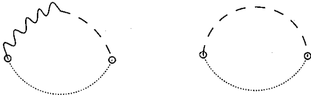
FIG. 1. The two graphs that contribute to C_{e^2} . Photon, \Phi_2 , and ghost propagators are indicated by wiggly, long-dashed, and short-dashed lines, respectively.
