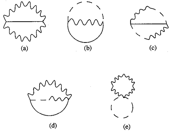
FIG. 3. The two-loop graphs that contribute to V_{e^2}^{\text{eff}} .
