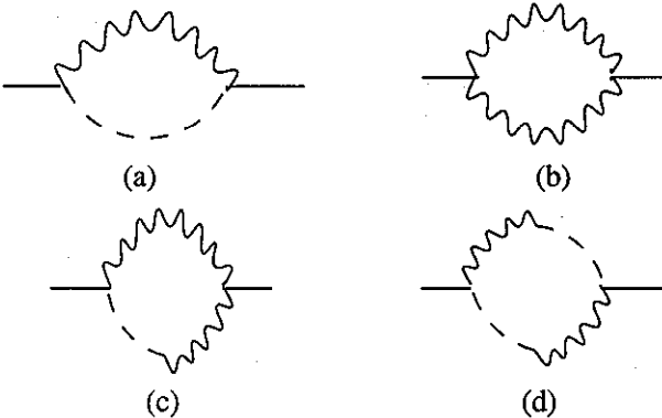
FIG. 2. The graphs that contribute to Z_{e^2} . Solid lines represent \Phi_1 propagators, with all other propagators shown as in Fig. 1.
