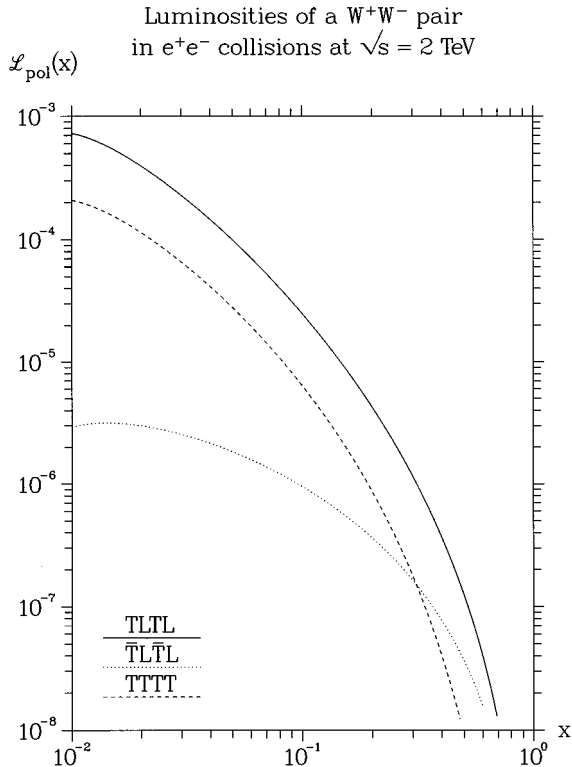
FIG. 3. Luminosities \mathcal{L}_{TLTL}(x) , \mathcal{L}_{\overline{TL}\overline{TL}}(x) , and \mathcal{L}_{TTTT}(x) for a W^+W^- pair in e^+e^- collisions at \sqrt{s}=2 TeV.
