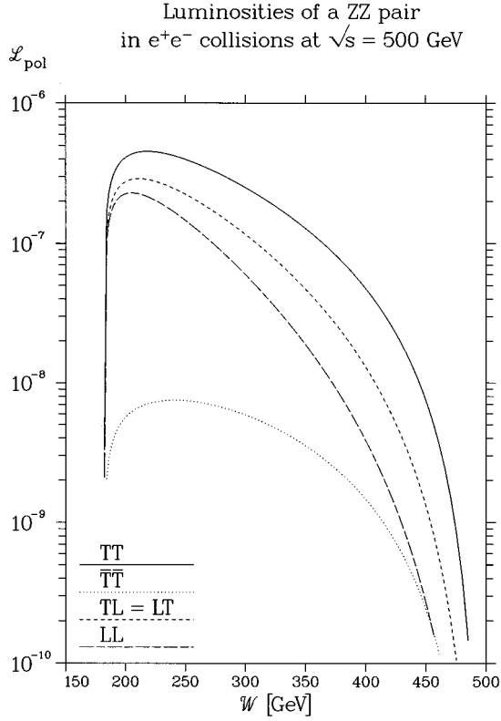
FIG. 9. Luminosities \mathcal{L}_{TT}(W) , \mathcal{L}_{\overline{TT}}(W) , \mathcal{L}_{LT}(W) , and \mathcal{L}_{LL}(W) for a ZZ pair in e^+e^- collisions at \sqrt{s} = 500 GeV.
