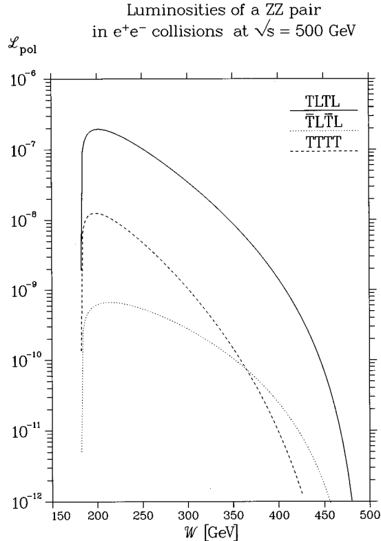
FIG. 10. Luminosities \mathcal{L}_{TLTL}(W) , \mathcal{L}_{\overline{TL}\overline{TL}}(W) , and \mathcal{L}_{TTTT}(W) for a ZZ pair in e^+e^- collisions at \sqrt{s} = 500 GeV.
