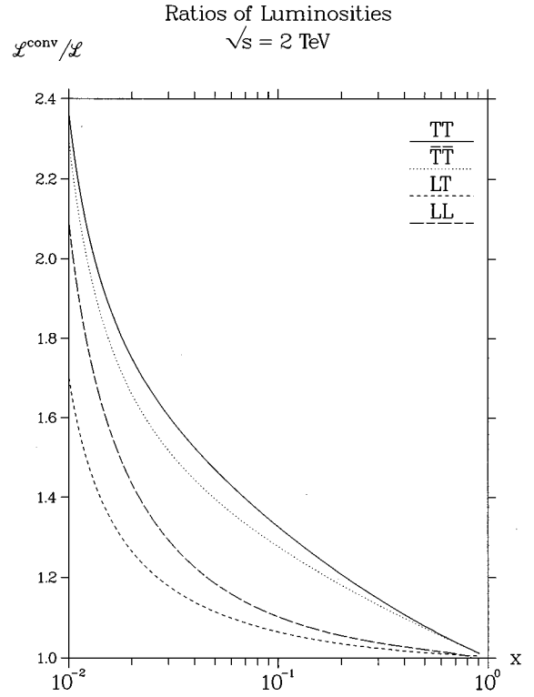
FIG. 4. Ratios of the convolutions of single-vector-boson distributions, Eq. (41), and the exact luminosities for \text{pol} = TT, \overline{TT}, LT , and LL for a W^+W^- pair in e^+e^- collisions at \sqrt{s}=2 TeV.
