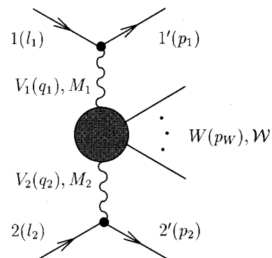
FIG. 1. The vector-boson scattering diagram.
