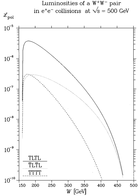
FIG. 8. Luminosities \mathcal{L}_{TLTL}(\mathcal{W}) , \mathcal{L}_{\bar{T}\bar{L}\bar{T}\bar{L}}(\mathcal{W}) , and \mathcal{L}_{TTTT}(\mathcal{W}) for a W^+W^- pair in e^+e^- collisions at \sqrt{s}=500 GeV.
