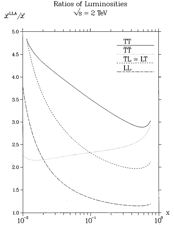
FIG. 6. Ratios of the leading logarithmic approximation for vector-boson pair luminosities, Eq. (45), and the exact luminosities for pol= TT , \overline{TT} , LT , and LL for a W^+W^- pair in e^+e^- collisions at \sqrt{s}=2 TeV.
