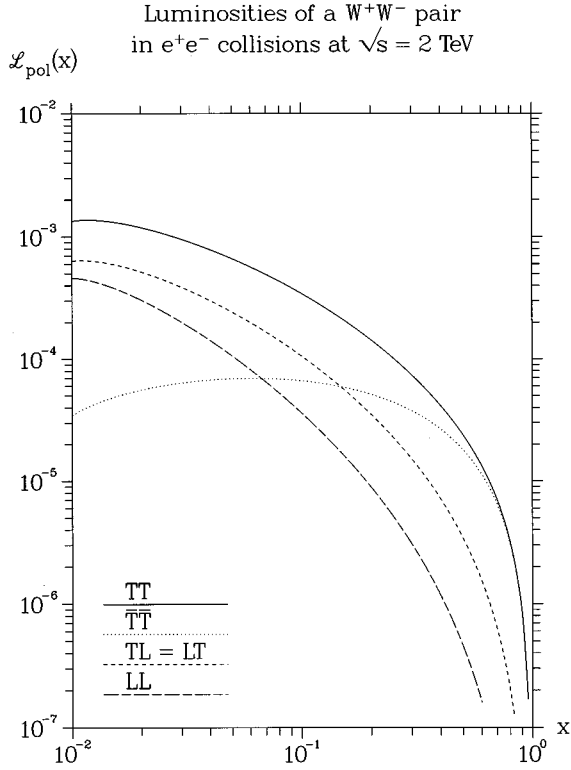
FIG. 2. Luminosities \mathcal{L}_{TT}(x) , \mathcal{L}_{\overline{TT}}(x) , \mathcal{L}_{LT}(x) , and \mathcal{L}_{LL}(x) for a W^+W^- pair in e^+e^- collisions at \sqrt{s}=2 TeV.
