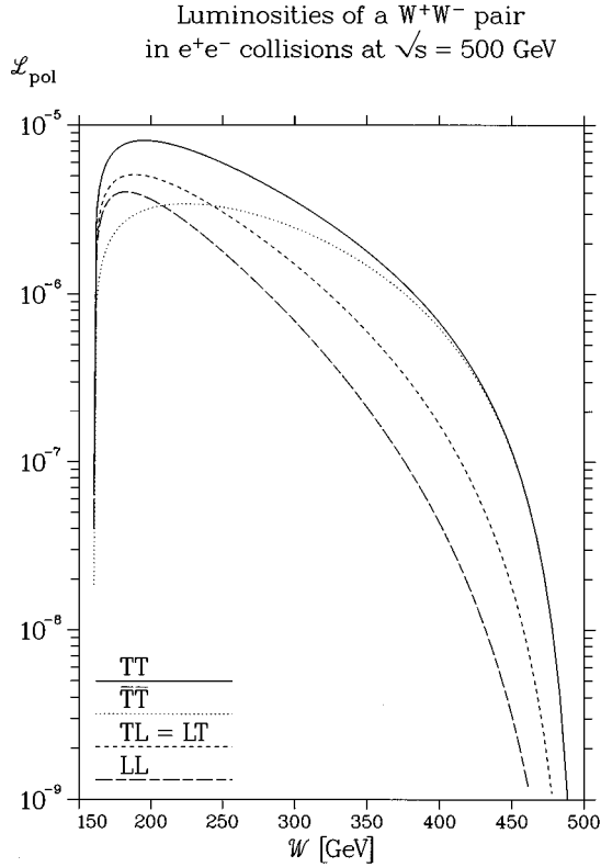
FIG. 7. Luminosities \mathcal{L}_{TT}(\mathcal{W}) , \mathcal{L}_{\bar{T}\bar{T}}(\mathcal{W}) , \mathcal{L}_{LT}(\mathcal{W}) , and \mathcal{L}_{LL}(\mathcal{W}) for a W^+W^- pair in e^+e^- collisions at \sqrt{s}=500 GeV.
