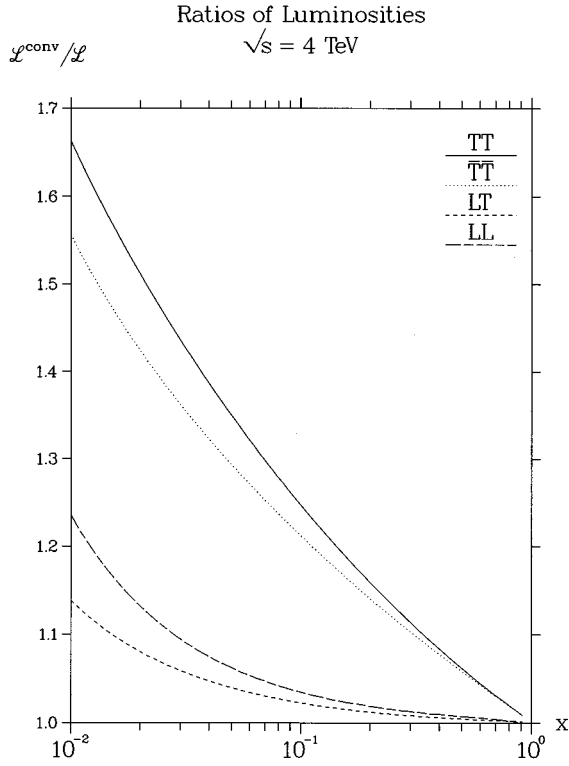
FIG. 5. Ratios of the convolutions of single-vector-boson distributions Eq. (41) and the exact luminosities for pol= TT , \overline{TT} , LT , and LL for a W^+W^- pair in e^+e^- collisions at \sqrt{s}=4 TeV.
