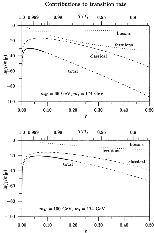
FIG. 3. Contributions to the transition rate \ln \gamma for fixed m_H = 66 GeV, m_t = 174 GeV, and m_H = 100 GeV, m_t = 174 GeV as a function of the parameter q = \sqrt{1 - T^2/T_c^2} . The total rate has a maximum close to the critical temperature. The region which mainly contributes to the integral Eq. (6.10) is marked by a solid line.
