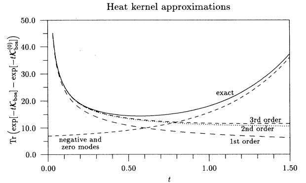
FIG. 1. Exact (solid line) and approximate values (dashed and dotted lines) of the heat kernel \text{Tr}(\exp[-t\mathcal{K}_{\text{bos}}] - \exp[-t\mathcal{K}_{\text{bos}}^{(0)}]) in dependence of the proper time parameter t . The exact result is obtained with the discretized spectrum of the fluctuation operator \mathcal{K}_{\text{bos}} , the approximations are the first 3 orders of the expansion in Eq. (7.1). For low t we obtain excellent agreement. The large t behavior of the heat kernel is governed by the negative and zero modes (dashed line).
