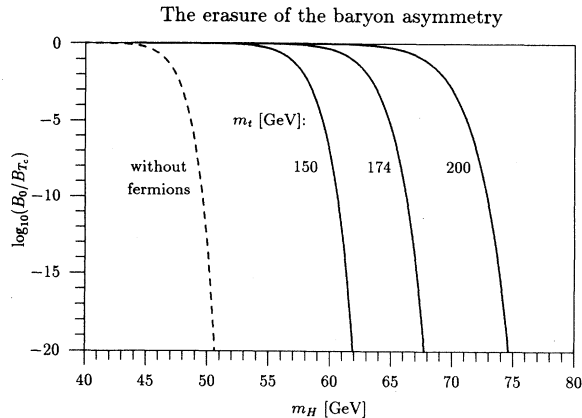
FIG. 5. The ratio B_0/B_{T_c} as a function of the Higgs boson mass m_H for m_t = 150, 174, and 200 GeV. From the condition that this ratio should be at least 10^{-5} we obtain an upper bound for m_H in the range 60 to 75 GeV. The same calculation without fermion loops leads to a qualitatively similar picture but the upper bound would be as low as 49 GeV.
