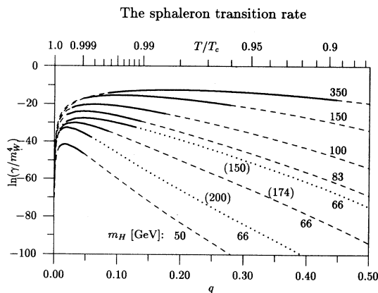
FIG. 4. The sphaleron transition rate \ln(\gamma/m_W^4) for various values of m_H (given without brackets) and m_t (given in brackets) depending on the parameter q = \sqrt{1 - T^2/T_c^2} . The dashed lines are for m_t = 174 GeV, the dotted lines for m_t = 150 and 200 GeV. The regions which mainly contribute to the baryon number violation are marked by solid lines.
