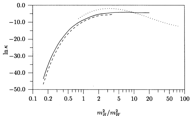
FIG. 2. \ln \kappa = -\beta_c E_{\text{bos}}^{\text{small}}(T_c) - \beta_c E_{\text{FP}}^{\text{small}}(T_c) - 6 \ln 2 - \ln |\omega_-| as a function of the Higgs mass. We compare our results (solid line) with those of Baacke et al. [16] (dashed line) and Carson et al. [15] (dotted line).
