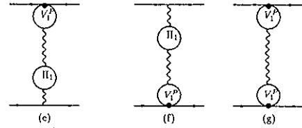
FIG. 2. The PT method applied to the scattering q\bar{q} \rightarrow q'q' at the two-loop QCD order.
