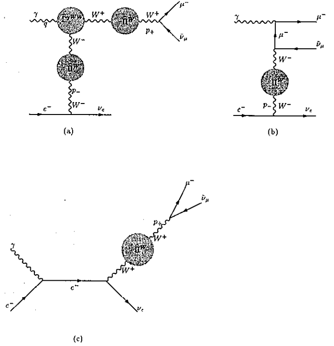
FIG. 8. The process e^- \gamma \rightarrow \mu^- \bar{\nu}_\mu \nu_e . The bubbles denote PT self-energies and three-point functions. Goldstone boson lines are not shown.
