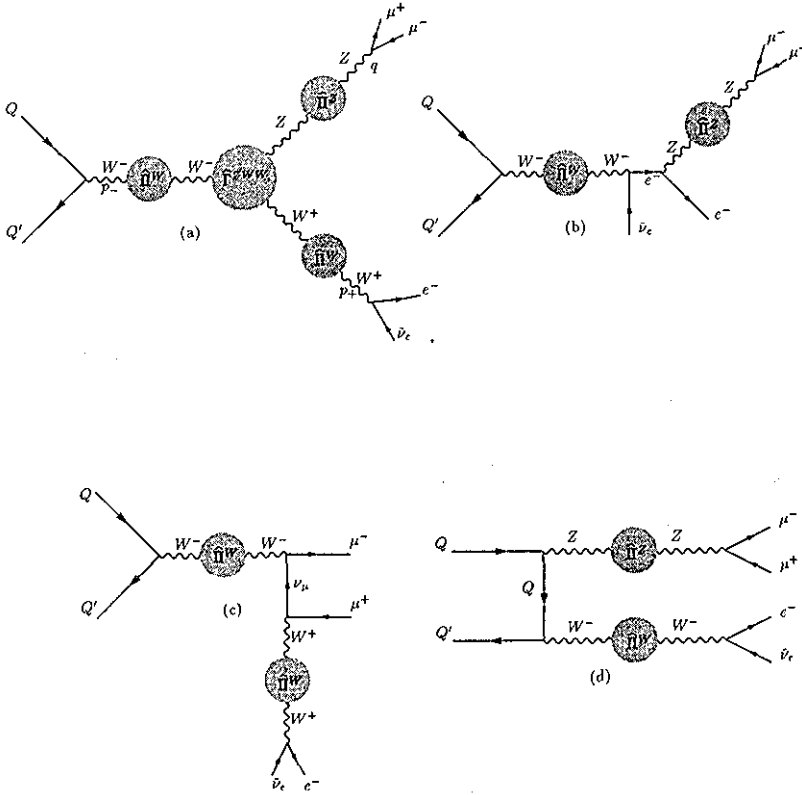
FIG. 9. The process QQ' \rightarrow \mu^+ \mu^- e^- \bar{\nu}_e , where Z\gamma -mixing effects and other photonic contributions are not shown. Crossed Z -boson exchange graphs are also implied.
