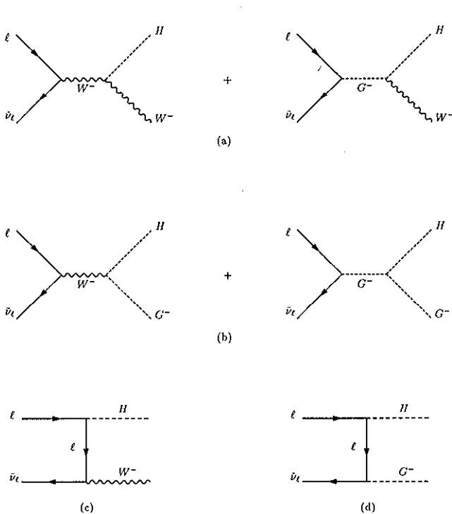
FIG. 6. The process l \bar{\nu}_l \rightarrow H W^- in an arbitrary R_t gauge.
