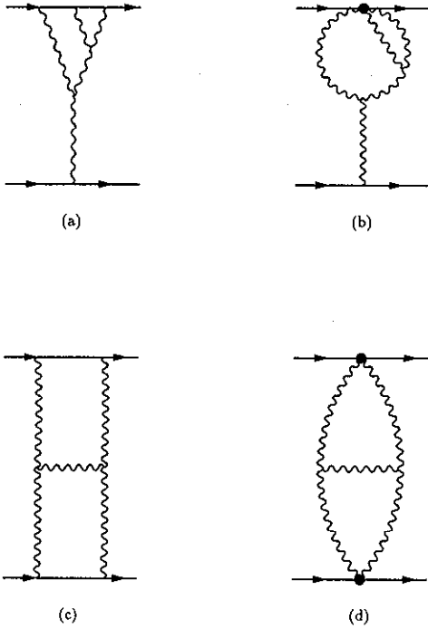
FIG. 4. Typical two-loop vertex and box graphs giving PT contributions to the two-loop PT self-energy.
