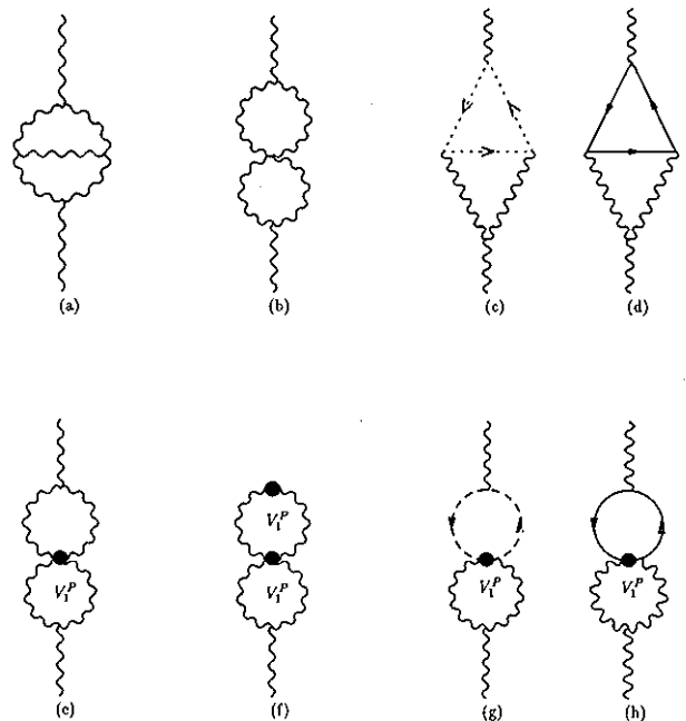
FIG. 3. Two-loop PT contributions to the gluon vacuum polarization.
