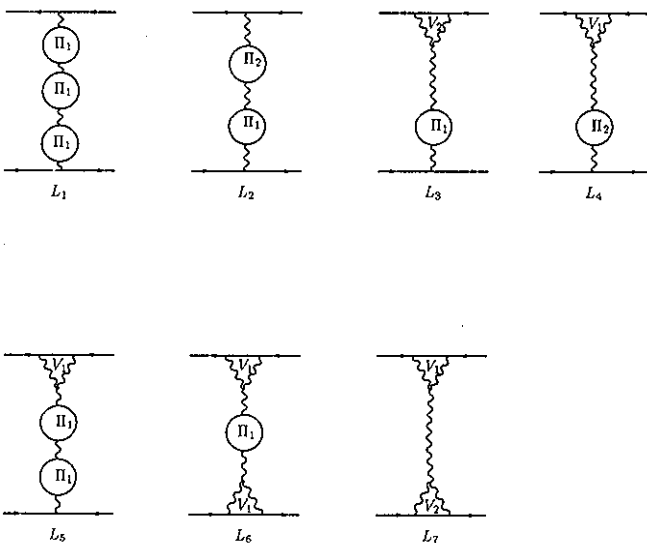
FIG. 10. Structures of Feynman graphs responsible for the vanishing of the shift of the pole at the three-loop case—see, also, Appendix A.
