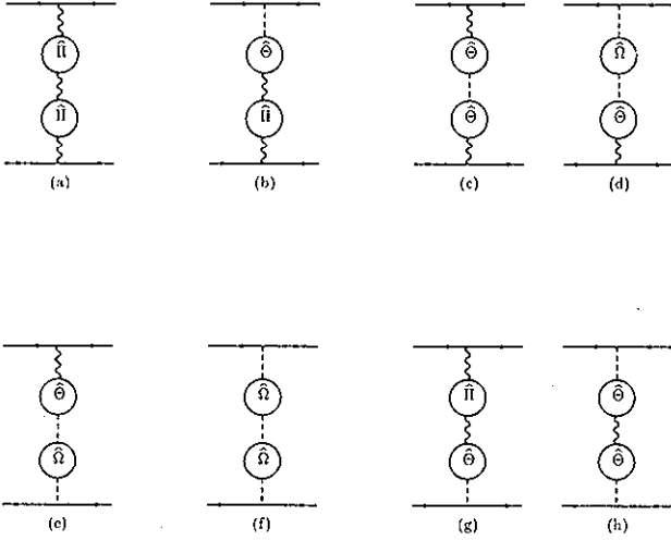
FIG. 5. The propagatorlike part \hat{T}_1 of the transition element for the process e^- \bar{\nu}_e \rightarrow \mu^- \bar{\nu}_\mu at the two-loop electroweak order.
