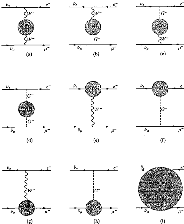
FIG. 1. The PT decomposition of the process e^-\bar{\nu}_e \rightarrow \mu^-\bar{\nu}_\mu (the arrow of time shows downwards).
