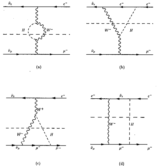
FIG. 7. The one loop absorptive graphs of the reaction e^- \bar{\nu}_e \rightarrow \mu^- \bar{\nu}_\mu involving the on-shell intermediate bosons W^- and H (the arrow of time shows downwards). Feynman lines with Goldstone bosons are not displayed.
