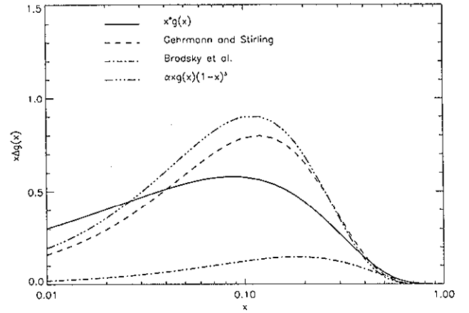
FIG. 5. Comparison of various polarized gluon distributions considered in the text.
