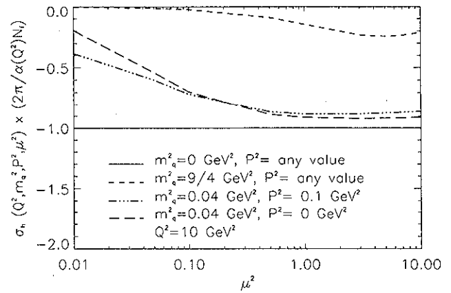
FIG. 2. Hard gluon coefficient as given by Eqs. (5), (7), and (12). The momentum transfer is fixed at 10 GeV 2 . It is seen that the strange quark contribution never equals that from the up and down quarks and the charm quark contribution is sizable for \mu^2 > 1 GeV 2 .
