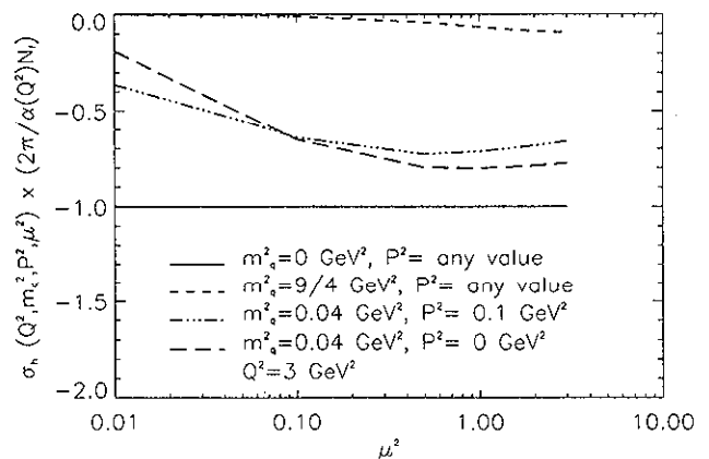
FIG. 3. Hard gluon coefficient as given by Eqs. (5), (7), and (12). The momentum transfer is fixed at 3 GeV 2 . It is seen that the strange quark contributes with approximately 75% of the up and down quarks in the realistic region of \mu^2 > 1 GeV 2 . In the same region, the charm quark gives a 10% contribution.
