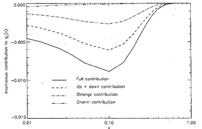
FIG. 6. Comparison of the x dependence of the non-strange, strange, and charm quark distributions to g_1(x) . The anomalous contribution is given by \frac{5}{36}\sigma_h^{\gamma^*g}(x, Q^2, \mu^2) \otimes \Delta g(x, \mu^2) and it is used in the form \Delta g(x, \mu^2 = 9 \text{ GeV}^2) = \alpha x g(x)(1-x)^3 for the polarized gluon.
