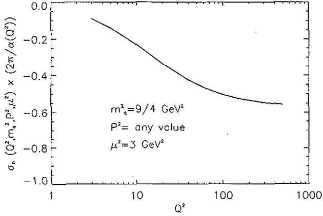
FIG. 4. Hard gluon coefficient for the charm quark, calculated with Eqs. (5), (7), and (12). The factorization scale is fixed at 3 GeV 2 and the Q^2 dependence is studied.
