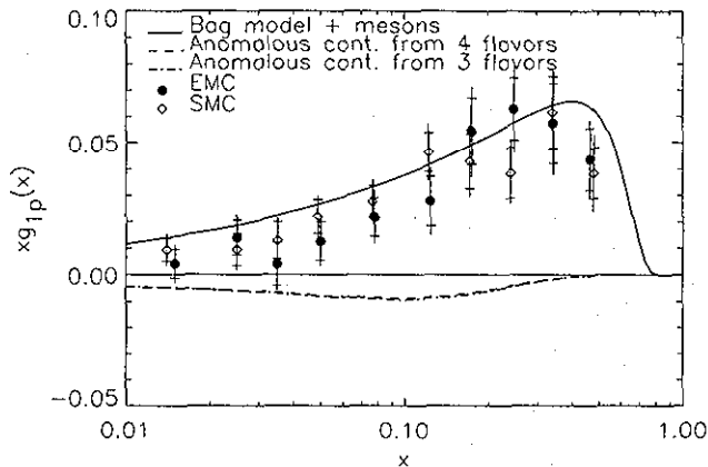
FIG. 7. EMC [15] and Spin Muon Collaboration (SMC) [16] data for g_{1p}^p(x) at 10 \text{ GeV}^2 . The theoretical curve for the polarized valence distribution is calculated in NLO and taken from Ref. [25]. The anomalous contribution should be subtracted from the theoretical curve.
