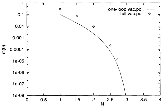
FIG. 4. The infrared mass m(0) with the one-loop vacuum polarization of massless fermions (solid line) and with the full vacuum polarization (diamonds), as a function of N .
