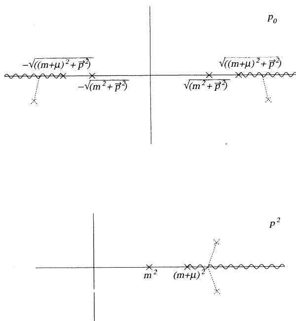
FIG. 1. The analytic structure of a full, stable, physical observable particle, in (a) the p_0 plane and (b) the p^2 plane (in Minkowski metric).
