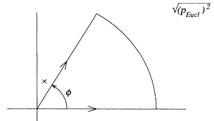
FIG. 2. The analytic continuation into the complex momentum plane of the integral equation (in Euclidean momenta).
