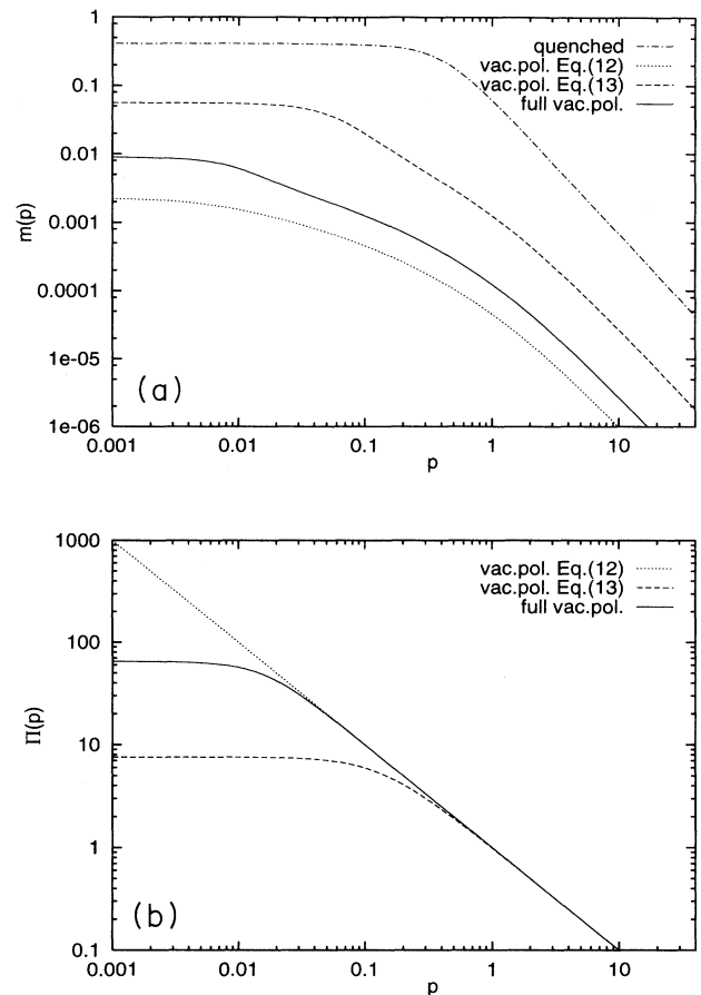
FIG. 7. The mass function (a) and vacuum polarization (b) as obtained by taking into account the one-loop vacuum polarization of massless fermions (dotted line), that of fermions with a fixed mass m(0) (dashed line), and that of dynamical fermions (solid line), all for N = 2 and in units of \alpha ; for completeness we included the mass function for quenched QED 3 (dashed-dotted line) in (a).
