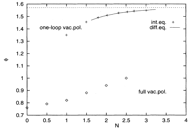
FIG. 5. The phase \phi of the mass singularity obtained with the one-loop vacuum polarization of massless fermions [both the results of using the integral equation Eq. (34) directly, and that of using a differential equation which can be derived from it, after some further approximations; see [23]], and with the full vacuum polarization (diamonds), as a function of N ; for completeness we have included the value for quenched QED 3 at N = 0 . The dotted line corresponds to \phi = \pi/2 , which means a mass singularity on the real timelike axis.
