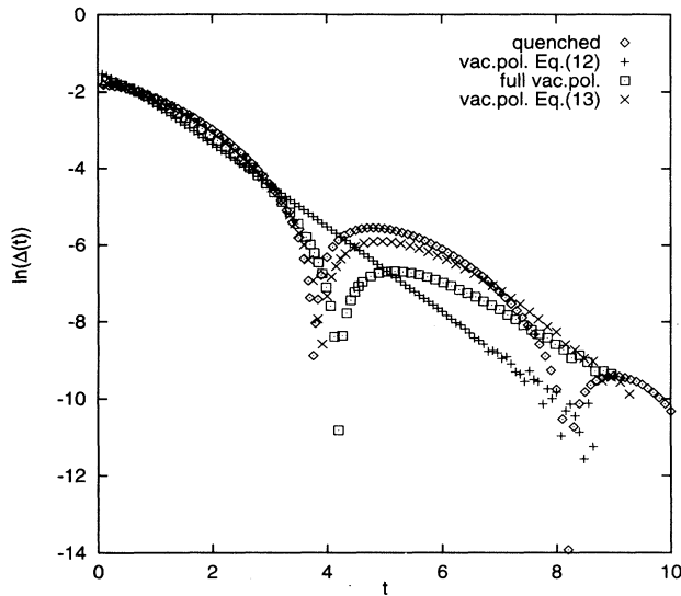
FIG. 6. The logarithm of the absolute value of the Schwinger function with N = 2 and some different approximations for the photon propagator: with the one-loop vacuum polarization of massless fermions [Eq. (12), pluses], with that of fermions with a fixed mass m(0) [Eq. (13), crosses], and with the full vacuum polarization with dynamical fermions (squares); for comparison, we also included the quenched results (diamonds).
