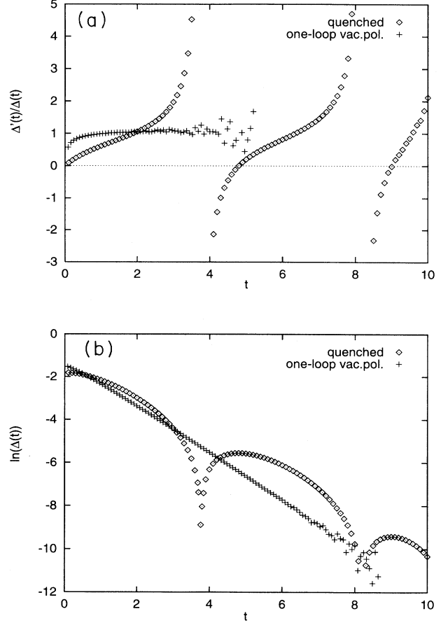
FIG. 3. The Schwinger function for quenched QED 3 ( N = 0 , diamonds) and with the one-loop vacuum polarization ( N = 2 , pluses): (a) the logarithmic derivative, (b) the logarithm of its absolute value; the energy scale is defined by requiring m(0) = 1 .
