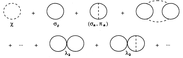
FIG. 2. Some neglected graphs. One-loop graphs subleading in 1/N ; and higher order graphs suppressed by powers of 1/N or \lambda_2 or both. Dashed lines are diagonalized \chi field propagators, solid lines are diagonalized \sigma and \pi fields.
