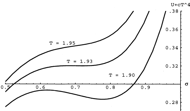
FIG. 3. The effective potential N^{-2}U(\sigma) for several temperatures, shifted by (\pi^2/45) T^4 for clarity, with all dimensionful quantities measured in units of v/N . A first order phase transition must occur below the temperature T_{\text{infect}} = 1.93v/N where the potential maximum and minimum coincide. The field strength discontinuity is at least 0.7v/N here, with parameters \lambda_1(M_r = 4.54v/N) = 40 = \lambda_2 .
