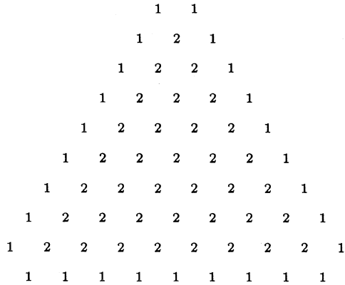
FIG. 3. Weight diagram for the SU(3) flavor representation of the spin- \frac{1}{2} baryons. The long side of the weight diagram contains \frac{1}{2}(N_c + 1) weights. The numbers denote the multiplicity of the weights.
