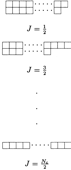
FIG. 2. SU(F) flavor representations for the tower of baryon states with J = \frac{1}{2}, \frac{3}{2}, \dots, \frac{N_c}{2} . Each Young tableau has N_c boxes.
