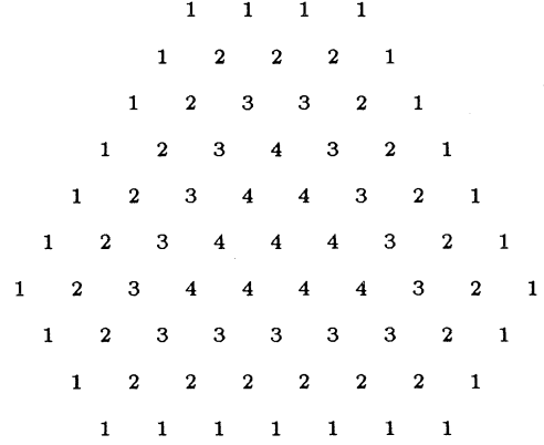
FIG. 4. Weight diagram for the SU(3) flavor representation of the spin- \frac{3}{2} baryons. The long side of the weight diagram contains \frac{1}{2}(N_c - 1) weights. The numbers denote the multiplicity of the weights.
