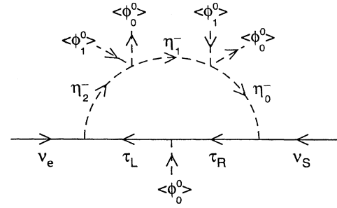
FIG. 1. One-loop radiative \nu_e - \nu_S mass due to the spontaneous breaking of the lepton number.
