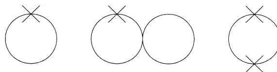
FIG. 2. Additional Feynman diagrams for the logarithm of the partition function in the effective theory.
