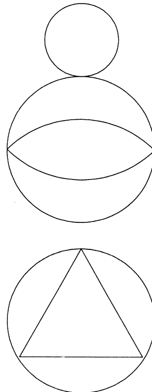
FIG. 5. Four-loop diagrams for the logarithm of the partition function of the effective theory which have logarithmic ultraviolet divergences.
