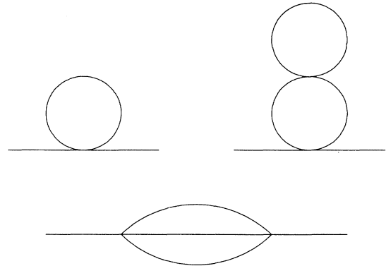
FIG. 3. Feynman diagrams for the self-energy in the full theory and in the effective theory.
