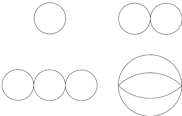
FIG. 1. Feynman diagrams for the logarithm of the partition function in the full theory and in the effective theory.
