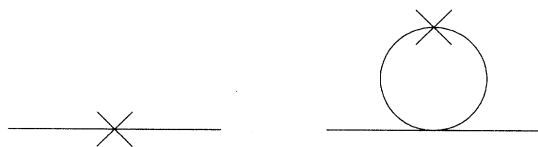
FIG. 4. Additional Feynman diagram for the self-energy in the effective theory.
