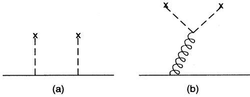
FIG. 3. (a) Graph contributing to the real part of the quasiparticle self-energy. The dashed lines represent either gluons, electroweak gauge bosons, or Higgs bosons from the plasma. These graphs are responsible for the thermal masses \Omega of the quasiparticles, shown in Fig. 1. (b) Graph describing a collision of a quasiparticle (solid line) with a quark or gluon (dashed line) in the plasma. This graph contributes to the imaginary part of the self-energy, and leads to the decoherence of quasiparticle waves.
