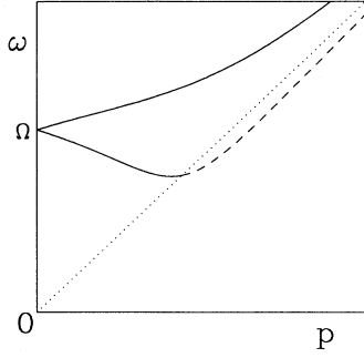
FIG. 1. Schematic picture of the dispersion relations for a fermionic quasiparticle in a hot plasma. The upper curve represents the normal branch. The lower curve represents the abnormal branch, which corresponds to the propagation of a “hole.” The abnormal branch becomes completely unstable when it passes through the light cone \omega = p (dotted line) [19].
