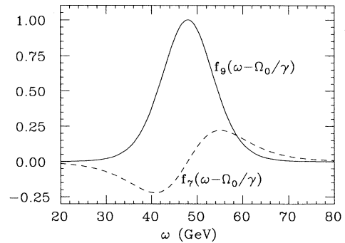
FIG. 5. The energy-dependent form factors f_7 and f_9 , evaluated at (\omega - \Omega_0)/\gamma = 6\ell(\omega - \Omega_0) . Note that f_9 is peaked at \omega = \Omega_0 \simeq 50 GeV, while f_7 vanishes there.
