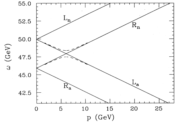
FIG. 2. Dispersion curves linearized for small momentum p . Because the W and Z bosons in the plasma only interact with left-handed quasiparticles, the dispersion relations for left-handed ( L ) and right-handed ( R ) quasiparticles are distinct. For a given chirality, the dispersion relations are as shown in Fig. 1, with both a normal branch ( n ) and an abnormal branch ( a ). (These curves are only shown for a single, light flavor. The curves for other light flavors would be shifted slightly in energy.) In the unbroken phase, the left-handed abnormal branch ( L_a ) intersects the right-handed normal branch ( R_n ); in the broken phase, the nonzero quark mass connects the two chiralities and level crossing occurs, as indicated by the dashed lines (here illustrated for the charm quark). The result is a mass gap with thickness of order the quark mass [7].
