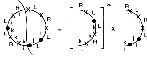
FIG. 6. This loop summarizes all the contributions to \Delta_9(\omega) , and corresponds to the trace in Eq. (65). [An analogous loop summarizes the contributions to \Delta_7(\omega) .] The solid blobs represent insertions of \delta p_L , which describes the mixing of quark flavors through interaction with the charged Higgs bosons. The crosses stand for insertions of the quark mass matrix. The loop is then a trace in flavor space of the product of all the insertions. Any individual contribution to the reflection asymmetry can be obtained by cutting across two segments of the loop of opposite chirality. This produces two open paths whose interference contributes to the asymmetry, as shown in the right side of the figure.
