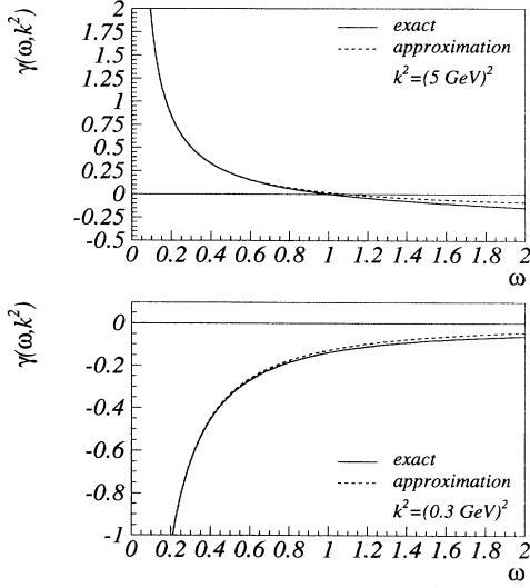
FIG. 6. Comparison between exact expression for the anomalous dimension (44) and the approximations (50) (top) and (51) (bottom).
