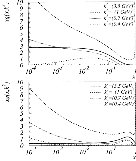
FIG. 7. Behavior of the distributions xg(x, k_{\perp}^2) of (56) and (57) for different values of k_{\perp}^2 . Top part shows result for a flat initial distribution xg(x, Q^2) = a(1-x)^c with a = 2.8 , c = 5.3 , and bottom part for a Gaussian initial distribution xg(x, Q^2) = 1/\sqrt{2\pi c^2} \exp[-(x-d)/(2c^2)] with c = 0.3 , d = 0.5 ( Q = 3.5 GeV, Q_0 = 1 GeV, \Lambda = 0.23 GeV).
