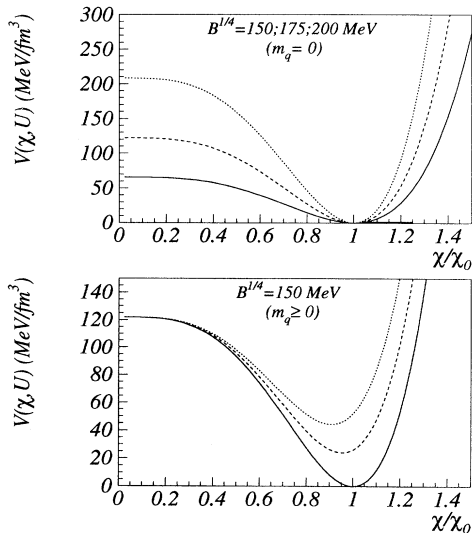
FIG. 1. Typical shape of V(\chi, U) , Eq. (14), with \partial V/\partial \chi = 0 at \chi = \chi_0 and V = B at \chi = 0 , where B = b\chi_0^4/4 is the bag constant.
