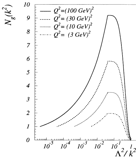
FIG. 8. Evolution of the gluon multiplicity N_g(k_{\perp}^2) from Q^2 down to \Lambda^2 . At first the gluons multiply, but at k_{\perp}^2 \approx Q_0^2 a condensation sets which is complete at \Lambda^2 ( Q_0 = 1 GeV, \Lambda = 0.23 GeV).
