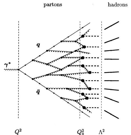
FIG. 2. Schematics of the parton shower evolution of a fragmenting q\bar{q} pair with its gluon configuration as the virtualities of the partons gradually degrade, starting from the hard scale Q^2 . At large gluon virtualities k^2 the shower develops by perturbative branching processes, but at k^2 \simeq Q_0^2 nonperturbative fusion and friction processes set in, such that at k^2 = \Lambda^2 no colored fluctuations remain.
