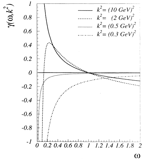
FIG. 5. The anomalous dimension \gamma(\omega, k_{\perp}^2) of Eq. (44) versus \omega for different values of k_{\perp}^2 .
