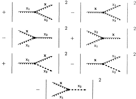
FIG. 4. Diagrams for the interaction probabilities that determine the evolution of the gluon distribution according to (38). In the probabilistic interpretation terms with positive signs lead to a gain of gluons and terms with negative sign to a loss. The gluon with momentum fraction x is the “observed” particle.
