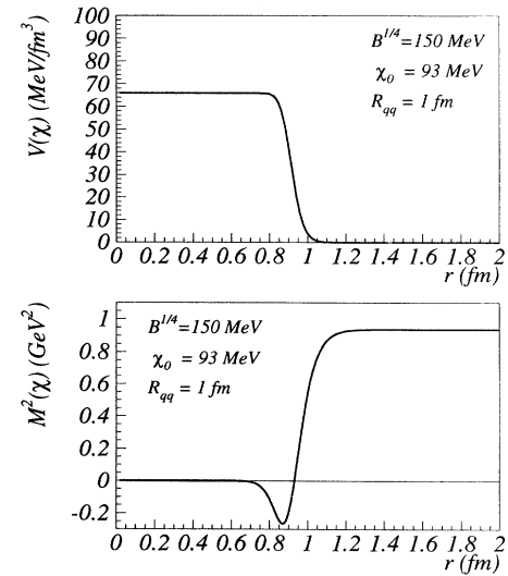
FIG. 10. (a) Form of the potential V[\chi(r)] and (b) the effective squared mass M^2[\chi(r)] of the \chi field, both at R_{q\bar{q}} = 1 fm ( \chi_0 = f_\pi and B^{1/4} = 150 MeV).
