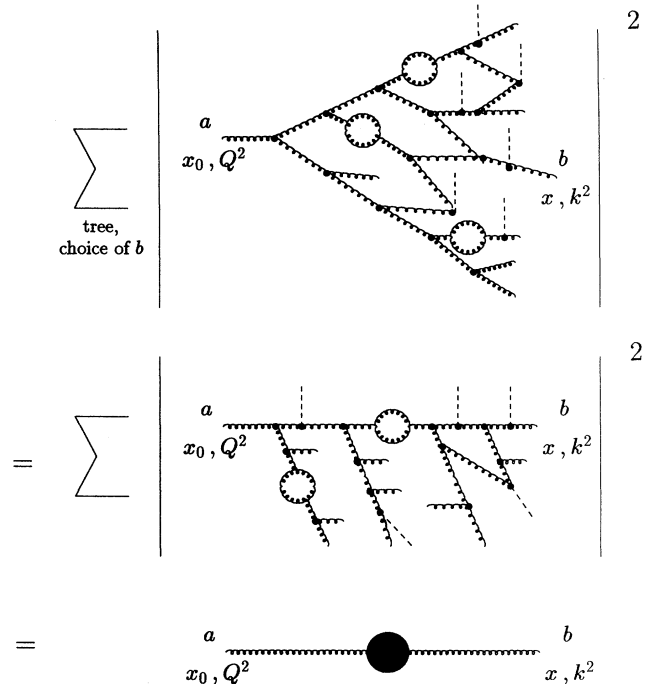
FIG. 3. Diagrammatic representation of the two-point Greens function of gluons, including both the gluon (self-)interactions and the effective interaction with the confining background field \chi (indicated by the dashed lines). This gluon propagator describes the evolution of a gluon from a chosen cascade branch in x and k^2 , starting from x_0 and Q^2 .
