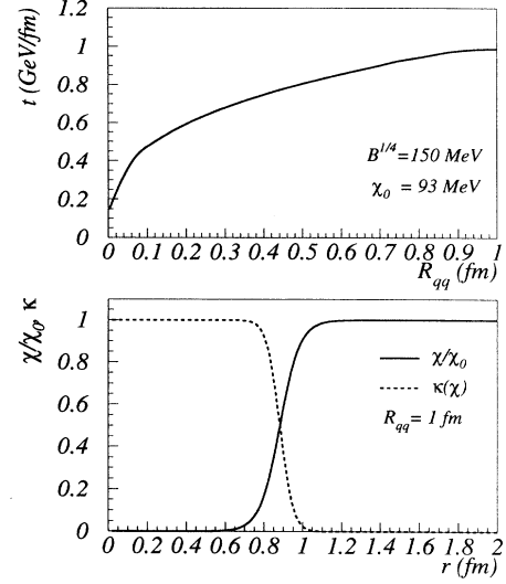
FIG. 9. (a) String tension t versus separation R_{q\bar{q}} of the q\bar{q} pair, and (b) the solutions for \chi and \kappa at R_{q\bar{q}} = 1 fm versus r which is the radial coordinate perpendicular to R_{q\bar{q}} ( \chi_0 = f_\pi and B^{1/4} = 150 MeV).
