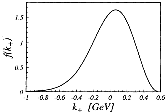
FIG. 3. Model ansatz (40) for the structure function f(k_+) , evaluated for \bar{\Lambda} = 0.57 GeV.
