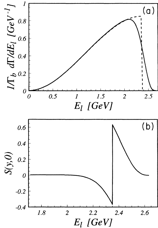
FIG. 5. Same as Fig. 4, but for B \rightarrow X_u \ell \bar{\nu} decays.
