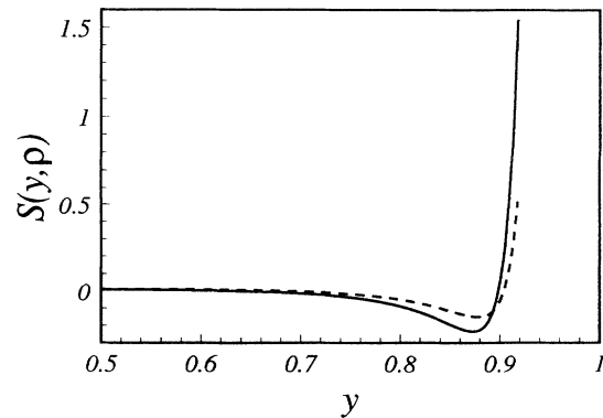
FIG. 2. Nonperturbative corrections to the lepton spectrum obtained using a naïve operator product expansion. The solid line corresponds to \lambda_1 = -0.3 \text{ GeV}^2 , the dashed one to \lambda_1 = -0.1 \text{ GeV}^2 .
