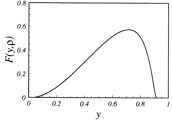
FIG. 1. Shape of the lepton spectrum predicted in the free-quark decay model. We use \rho = (m_c/m_b)^2 = 0.08 .
