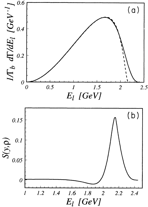
FIG. 4. (a) Charged-lepton spectrum (1/\Gamma_b) d\Gamma/dE_\ell in B \rightarrow X_c \ell \bar{\nu} decays. The solid line is obtained from the convolution in (33) using the ansatz (40) for the structure function. The dashed line shows the prediction of the free-quark decay model. (b) The shape function S(y, \rho) , which is obtained from the difference of the two curves in (a).
