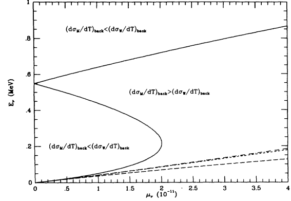
FIG. 2. Regions of dominance of weak or magnetic backward differential cross sections in the plane (\mu_\nu, E_\nu) for \bar{\nu}_e ; there are three different zones divided by the solid line. For the rest of (anti)neutrinos there are only two regions, the magnetic backward cross sections being dominant below the corresponding line (long-dashed for \nu_e , dash-dotted for \bar{\nu}_\mu , and short-dashed for \nu_\mu ) and the opposite above the line.
