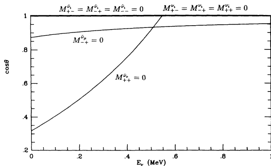
FIG. 1. Kinematical and dynamical zeros for the helicity amplitudes in the plane (E_\nu, \cos\theta) . The kinematical ones correspond to the line \cos\theta=1 . The curves have been done for \sin^2\theta_W=0.233 .
