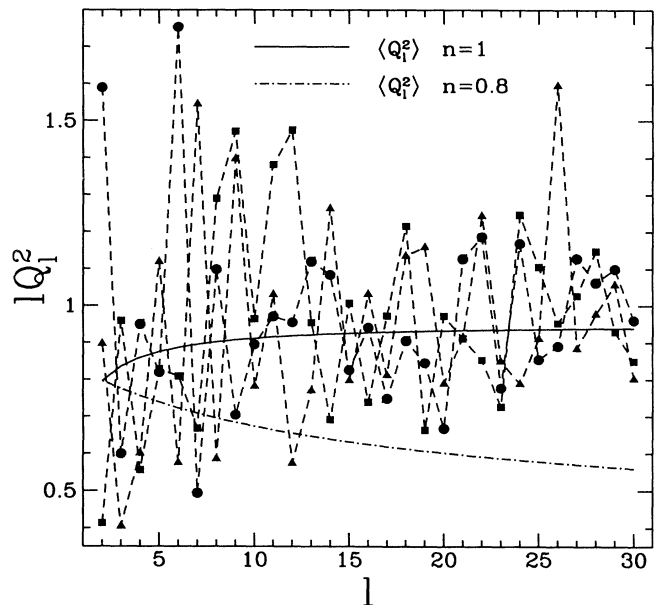
FIG. 2. Multipoles up to l=30 , roughly corresponding to the complete range of large scales. The solid line represents the ensemble averaged \langle Q_l^2 \rangle (multiplied by l ) for a flat ( n=1 ) spectrum of scalar density perturbations with A_G(\lambda) \ll A_S(\lambda) , normalized to \Sigma_2^2=1 . The three dashed lines represent different randomly chosen realizations of this distribution. Observations can only supply one such line, giving little clue to the ensemble average quantity that inflation supplies the form of. For comparison, the dash-dotted line shows the result of a scalar spectrum with n=0.8 , again with A_G(\lambda) \ll A_S(\lambda) (such a combination would arise from an appropriate inverted harmonic oscillator potential). Note that the normalization of this line is arbitrary (shown here with \Sigma_2^2=1 ), and were it moved up it could match an observed distribution across much of the range. More significantly, it is easy to note that any detailed information in the spectrum such as peaks or troughs can be swamped completely by the cosmic variance.
