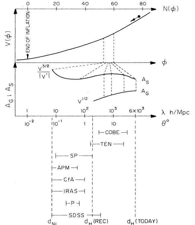
FIG. 1. A schematic figure illustrating the main concepts behind reconstruction. For inflation the two main steps involve converting the observations (lower half of figure) into the primordial scalar ( A_S ) and tensor ( A_G ) fluctuation spectra and then working in reverse to reconstruct the potential V(\phi) . The main observational information from the cosmic microwave background arises through the Cosmic Background Explorer (COBE) satellite [1], and the Tenerife (TEN) [48] and South Pole (SP) [50] collaborations. Galaxy surveys (APM [41], CfA [34], and IRAS [39,40]) may provide useful information up to 100h^{-1} Mpc, while the Sloan Digital Sky Survey (SDSS) [32] should extend to the lowest scales measured by COBE. Peculiar velocity measurements using the POTENT (P) [42] methods are important on intermediate scales. The angle \theta measures angular scales on the CMBR in degrees, and length scales \lambda are in units of h^{-1} Mpc. d_H refers to the horizon size today and at recombination and d_{\text{NL}} \approx 8h^{-1} Mpc is the scale of nonlinearity. (See the text for details.) Perfect observations will only reconstruct a small portion of the inflaton potential corresponding to between 53 \leq \Delta N \leq 60 e -foldings before the end of inflation.
