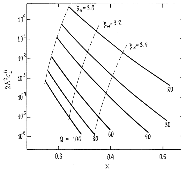
FIG. 2. Cross section in (2.20) as a function of Bjorken x = Q^2/(2pq) for different values of Q (solid curves). The dashed curves show the lines with the constant saddle-point value of the conformal parameter \xi_* .
