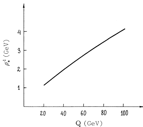
FIG. 4. Saddle-point value of the instanton size \rho_* as a function of Q and for \xi_* \sim 3\text{--}4 . The dependence on \xi_* is actually very weak.
