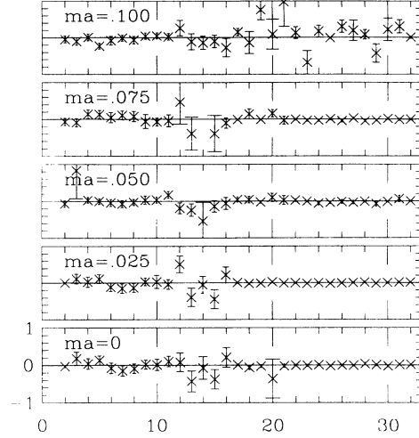
FIG. 1. Expectation value of various hypercube meson fields at \beta = 5.10 vs operator index. The i th operator is \pi_i for i = 1, 2, \dots, 16 and is \bar{\pi}_{i-16} for i = 17, \dots, 32 . The expectation value of the i = 1 operator, the \sigma meson, is given separately in Table IV. All values should be multiplied by 10^{-2} .
