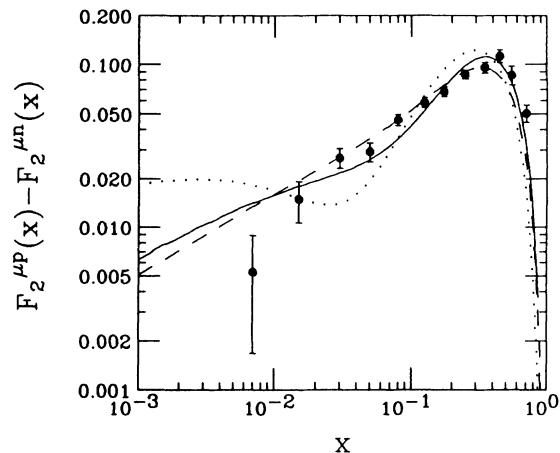
FIG. 2. NMC measurements of the difference F_2^{\mu p}(x) - F_2^{\mu n}(x) vs x , Ref. [1]. Solid curve: modified EHLQ structure functions, Eq. (6); dotted curve: HMRS(EB) structure functions, Ref. [6]; dashed curve: chiral field theory.
