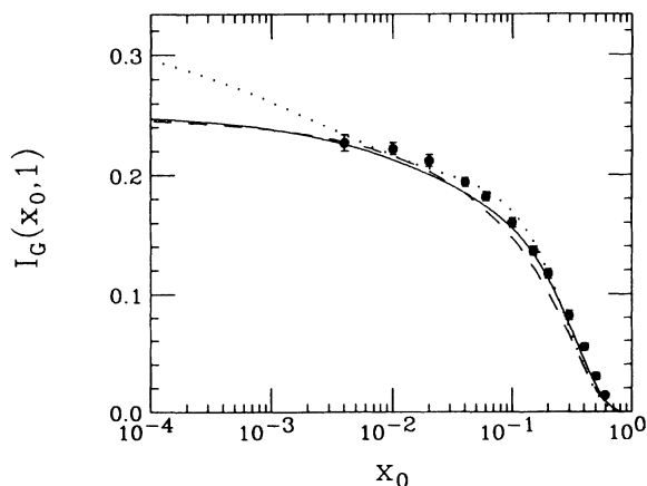
FIG. 1. Gottfried-sum-rule integral I_G(x_0, 1) vs x_0 , measured by the New Muon Collaboration, Ref. [1]. Solid curve: modified EHLQ structure functions, Eq. (6); dotted curve: HMRS(EB) structure functions, Ref. [6]; dashed curve: chiral field theory.
