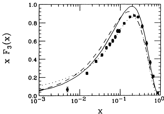
FIG. 3. Preliminary data of the CCFR Collaboration on the structure function x\mathcal{F}_3^{\nu N}(x) at Q^2 = 3 \text{ GeV}^2 , Ref. [12]. Solid curve: modified EHLQ structure functions, Eq. (6); dotted curve: HMRS(EB) structure functions, Ref. [6]; dashed curve: chiral field theory.
