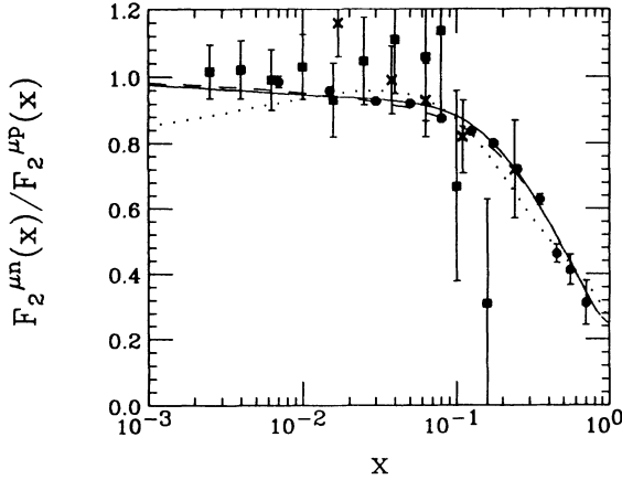
FIG. 4. NMC measurements (●) of the ratio F_2^{\mu n}(x)/F_2^{\mu p}(x) vs x , Ref. [1]. Solid curve: modified EHLQ structure functions, Eq. (6); dotted curve: HMRS(EB) structure functions, Ref. [6]; dashed curve: chiral field theory. Also shown (■ and ×) are preliminary data of Fermilab Experiment E-665, from Ref. [7].
