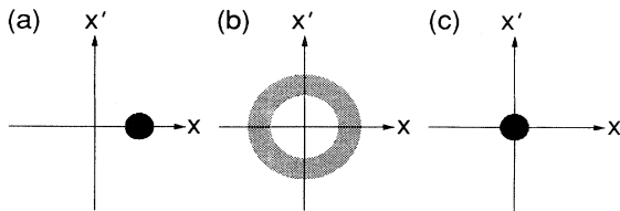
FIG. 1. Phase space of a bunch (a) upon injection with a coherent oscillation, (b) after decoherence due to a tune spread, and (c) after synchrotron radiation has damped the incoherent oscillations.
