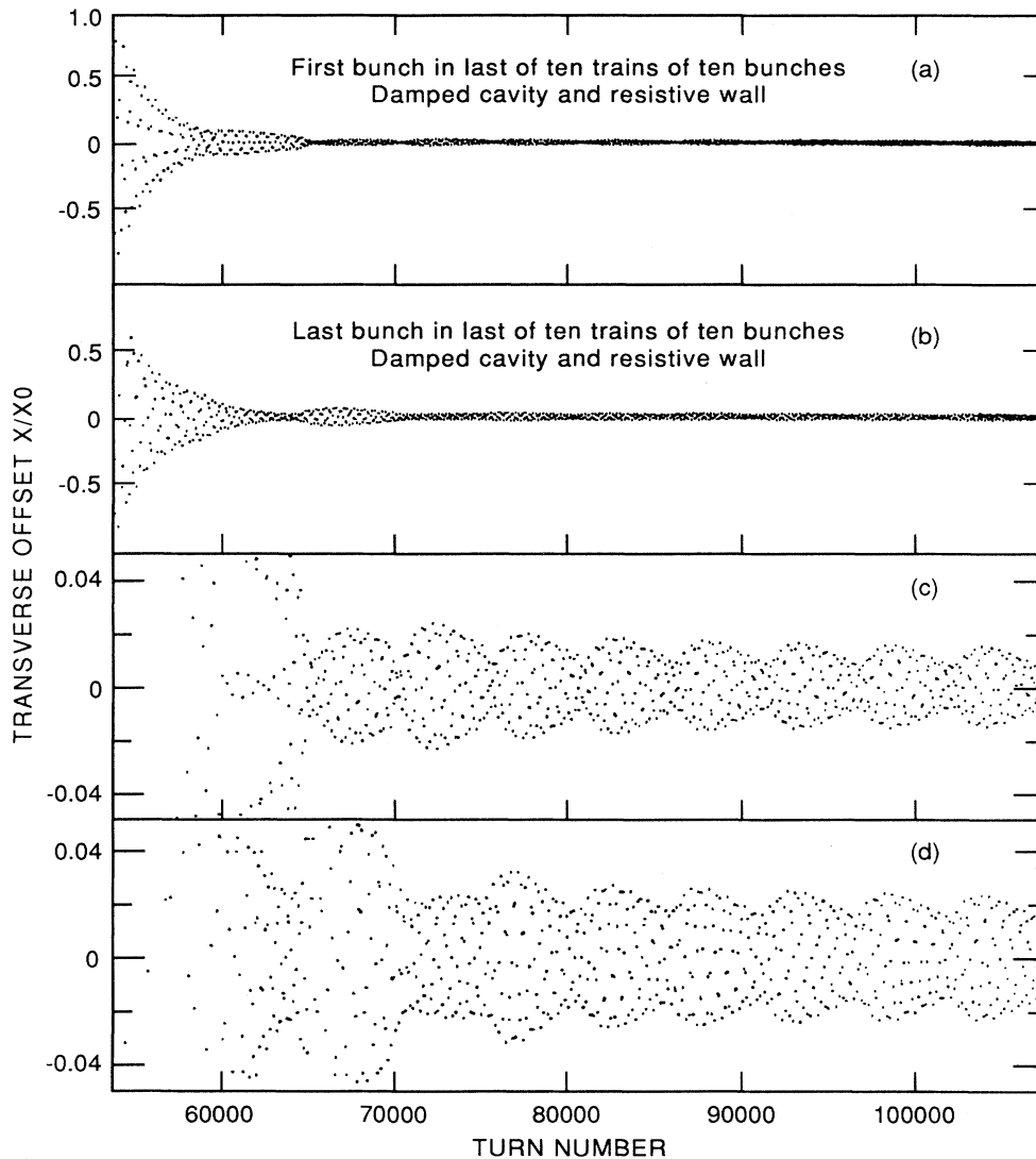
FIG. 4. Transverse bunch offset (divided by x_0 ) vs turn number for (a) the first bunch, and (b) the last bunch, in the last of ten trains of ten bunches, including the mode-damped-cavity and resistive-wall wakes. The coherent damping assumed is \zeta=900 \text{ s}^{-1} . Parts (c) and (d) are the same as parts (a) and (b), respectively, except for an expanded vertical scale.
