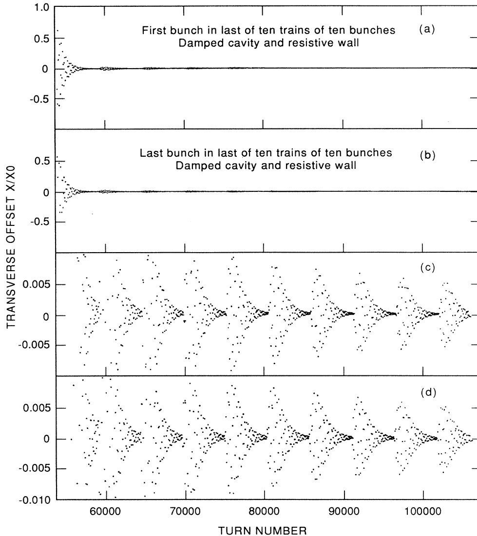
FIG. 5. Transverse bunch offset (divided by x_0 ) vs turn number for (a) the first bunch, and (b) the last bunch, in the last of ten trains of ten bunches, including the mode-damped-cavity and resistive-wall wakes. The coherent damping assumed is \zeta=2500 \text{ s}^{-1} . Parts (c) and (d) are the same as parts (a) and (b), respectively, except for an expanded vertical scale.
