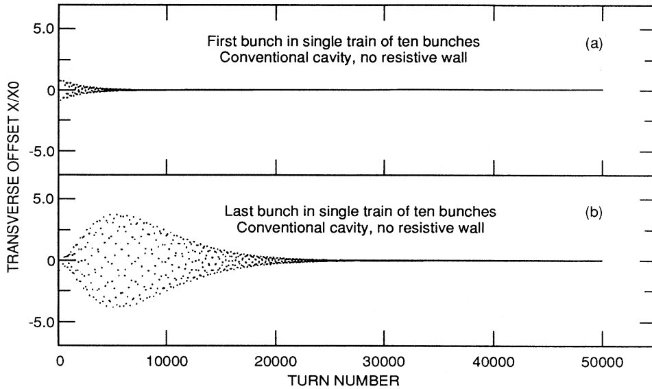
FIG. 2. Transverse bunch offset (divided by the initial offset x_0 of the bunches) vs turn number for (a) the first bunch, and (b) the last bunch in a single train of ten bunches, assuming the conventional cavity design and no resistive wall wake. The coherent damping assumed is \zeta = 900 \text{ s}^{-1} .
