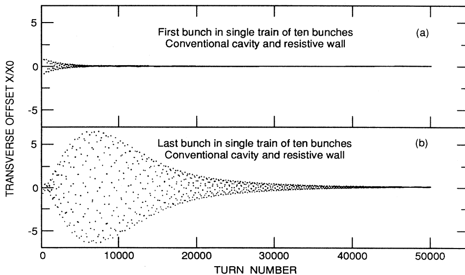
FIG. 3. Transverse bunch offset (divided by x_0 ) vs turn number for (a) the first bunch, and (b) the last bunch in a single train of ten bunches, assuming the conventional cavity design and a resistive wall wake. The coherent damping assumed is \zeta = 900 \text{ s}^{-1} .
