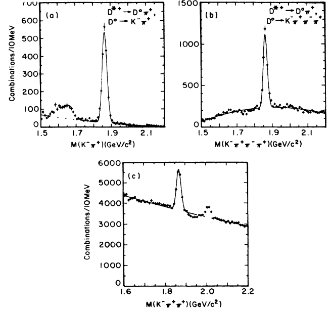
FIG. 1. Invariant-mass spectra: D^{*+} and D^+ candidates with x_p > 0.6 . (a) m(K^-\pi^+) with cut on D^{*+} - D^0 mass difference, (b) m(K^-\pi^+\pi^-\pi^+) with cut on D^{*+} - D^0 mass difference, and (c) m(K^-\pi^+\pi^+) .
