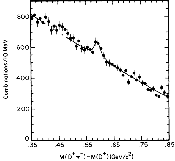
FIG. 2. The m(D^+\pi^-)-m(D^+) mass-difference spectrum with fit for the D^{**0}(2461) signal.
