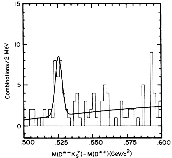
FIG. 7. The m(D^{*+}K_S^0) - m(D^{*+}) mass-difference spectrum.
