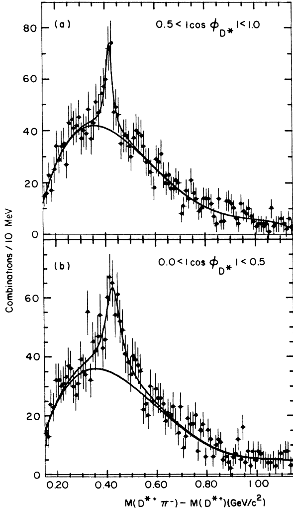
FIG. 4. The m(D^{*+}\pi^-) - m(D^{*+}) mass-difference spectra, (a) 0.5 < |\cos\phi_{D^*}| < 1.0 and (b) 0.0 < |\cos\phi_{D^*}| < 0.5 . We use a Breit-Wigner distribution to fit the signal and fourth-order Chebyshev polynomial to fit the background.
