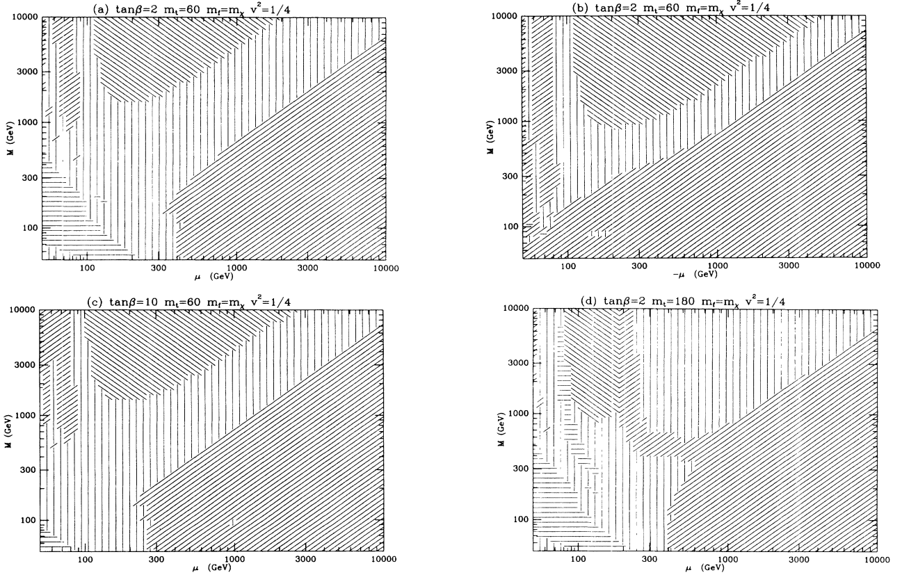
FIG. 6. Hatch plots that illustrate the importance of the various channels for neutralino annihilation in the early Universe ( v^2 \approx \frac{1}{4} ). In the areas “hatched” with positively sloped lines, annihilation into fermion final states dominates by at least a factor of 10; in the regions marked by negatively sloped lines, annihilation into gauge-boson final states dominates by at least a factor of 10; and in the regions hatched with horizontal lines, annihilation into Higgs-boson final states dominates by at least a factor of 10. In the regions hatched by vertical lines, several final states contribute comparably to the annihilation. Here m_{\tilde{f}} = m_{\tilde{\chi}} is used throughout. The values of m_t and \tan\beta , and the sign of \mu are as indicated. Hatch plots for other values of m_t and \tan\beta are qualitatively similar.
