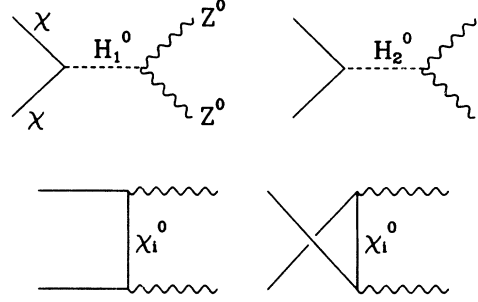
FIG. 3. Feynman diagrams for neutralino annihilation into ZZ final states. The index i runs from 1 to 4.
