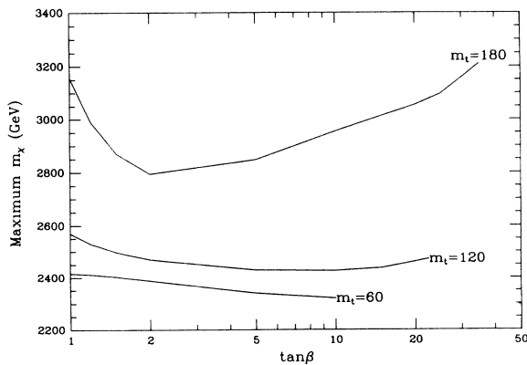
FIG. 14. Cosmological upper bound to m_{\tilde{\chi}} as a function of \tan\beta for several values of the top-quark mass.
