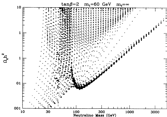
FIG. 17. Same as Fig. 15(a) with m_{\tilde{f}} = \infty .
