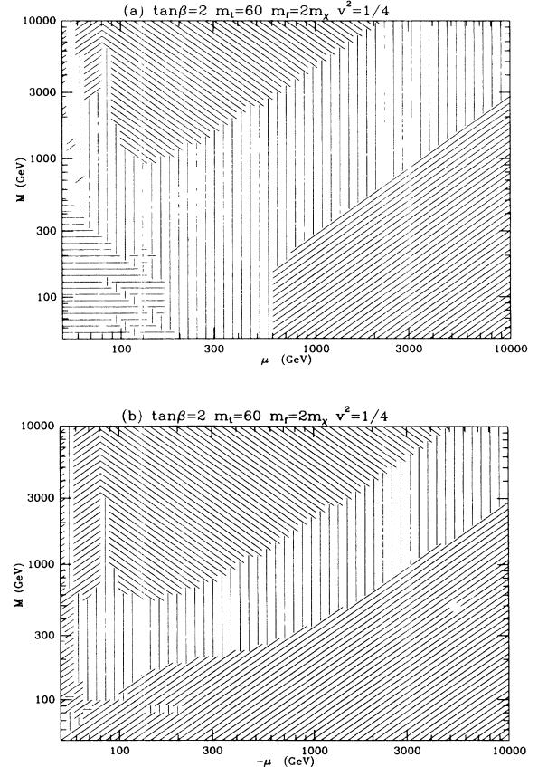
FIG. 7. Same as Fig. 6(a) but with m_{\tilde{f}} = 2m_{\tilde{\chi}} .
