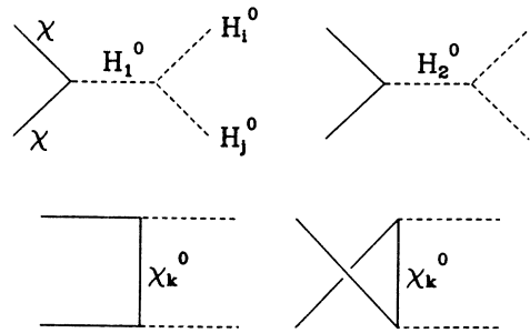
FIG. 4. Feynman diagrams for neutralino annihilation into H_i^0H_j^0 final states where c_i = c_j . There are a total of ten diagrams since the index k runs from 1 to 4.
