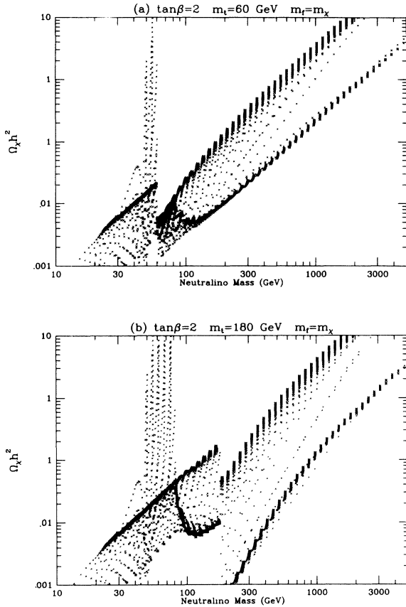
FIG. 15. Scatter plots of \Omega_{\tilde{\chi}} h^2 vs neutralino mass for a wide range of models (assuming m_{\tilde{f}} = m_{\tilde{\chi}} and \tan\beta = 2 ). In (a) we use m_t = 60 GeV, and in (b) we use m_t = 180 GeV. Each \times represents a different supersymmetric model specified by the value of \mu and M . The values selected for M and \mu were taken from a grid on the M - \mu plane. Results for other values of \tan\beta are qualitatively similar.
