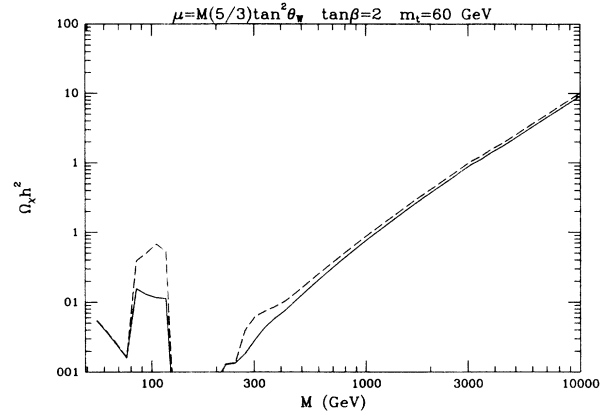
FIG. 11. Relic neutralino abundance as a function of M for \mu = \frac{5}{3} M \tan^2 \theta_w , \tan\beta=2 and m_t=60 GeV. Again the solid line shows \Omega_{\tilde{\chi}} h^2 assuming m_{\tilde{f}} = m_{\tilde{\chi}} , and the broken line shows \Omega_{\tilde{\chi}} h^2 assuming m_{\tilde{f}} = \infty . Again we have taken \tan\beta=2 and m_t=60 GeV. Plots for \mu < 0 and other values of \tan\beta and m_t are similar.
