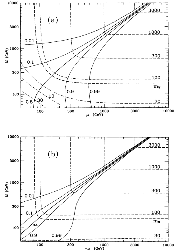
FIG. 1. Lightest neutralino composition and mass for \tan\beta = 2 . The broken curves are contours of constant neutralino mass m_{\tilde{\chi}} , and the solid curves are contours of constant gaugino fraction ( Z_{n1}^2 + Z_{n2}^2 ); in (a) \mu > 0 and in (b) \mu < 0 .
