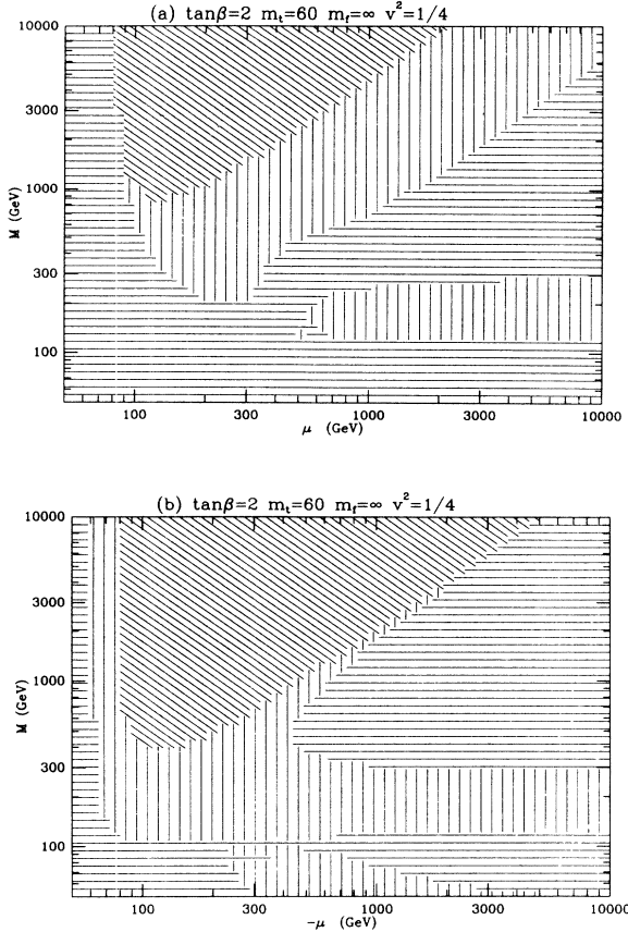
FIG. 8. Same as Fig. 6(a) but with m_{\tilde{f}} = \infty .
