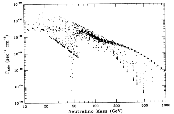
FIG. 18. Scatter plot of estimated halo annihilation rate vs neutralino mass for a wide range of models (assuming m_{H_2^0} = 0 , \tan\beta = 2 , m_t = 60 , and using m_{\tilde{f}} = m_{\tilde{\chi}} or m_{\tilde{f}} = \infty ).
