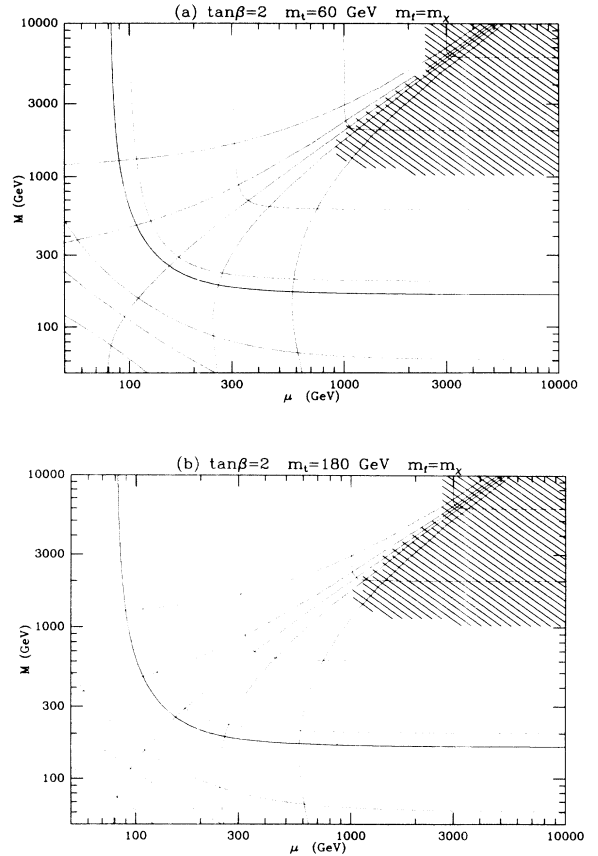
FIG. 12. Cosmologically excluded regions of the M - \mu plane for several values of m_t using \tan\beta=2 . The hatched areas are those for which \Omega_{\tilde{\chi}} h^2 > 1 independent of m_{H_2^0} and m_{\tilde{f}} . Plots for \mu < 0 and other values of \tan\beta are very similar.
