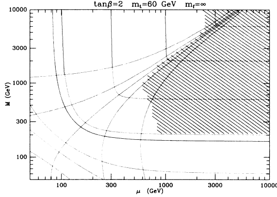
FIG. 13. Same as Fig. 12(a) but assuming m_f = \infty .
