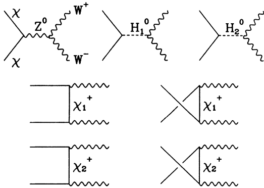
FIG. 2. Feynman diagrams for neutralino annihilation into W^+W^- final states.
