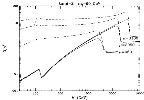
FIG. 9. Relic neutralino abundance as a function of M for several fixed values of \mu . The solid curves show \Omega_{\tilde{\chi}} h^2 assuming m_{\tilde{f}} = m_{\tilde{\chi}} , and the broken curves show \Omega_{\tilde{\chi}} h^2 assuming m_{\tilde{f}} = \infty . Here we have taken \tan\beta=2 and m_t=60 GeV. Results for \mu < 0 and other values of \tan\beta and m_t are qualitatively similar.
