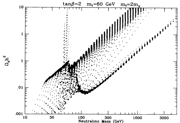
FIG. 16. Same as Fig. 15(a) with m_{\tilde{f}} = 2m_{\tilde{\chi}} .
