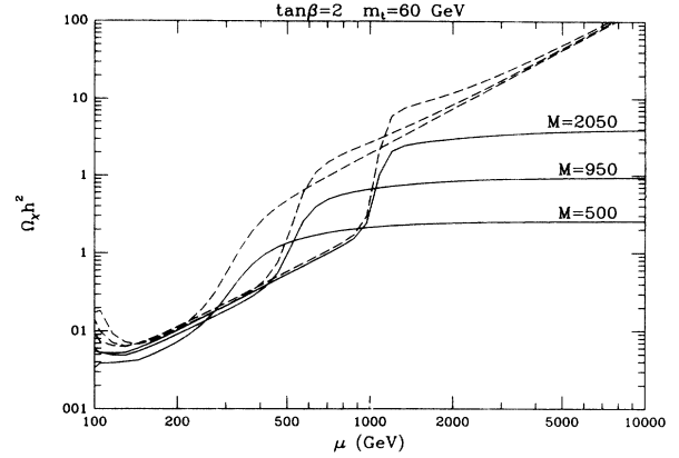
FIG. 10. Relic neutralino abundance as a function of \mu for several fixed values of M . Again the solid curves show \Omega_{\tilde{\chi}} h^2 assuming m_{\tilde{f}} = m_{\tilde{\chi}} , and the broken curves show \Omega_{\tilde{\chi}} h^2 assuming m_{\tilde{f}} = \infty for the same three values of M . Again we have taken \tan\beta=2 and m_t=60 GeV. Results for \mu < 0 and other values of \tan\beta and m_t are qualitatively similar.
