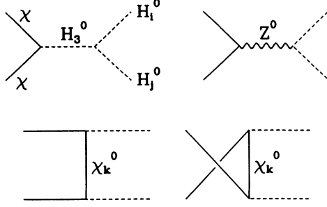
FIG. 5. Feynman diagrams for neutralino annihilation into H_i^0 H_j^0 final states where c_i \neq c_j ( H_2^0 H_3^0 and H_1^0 H_3^0 only). The index k runs from 1 to 4.
