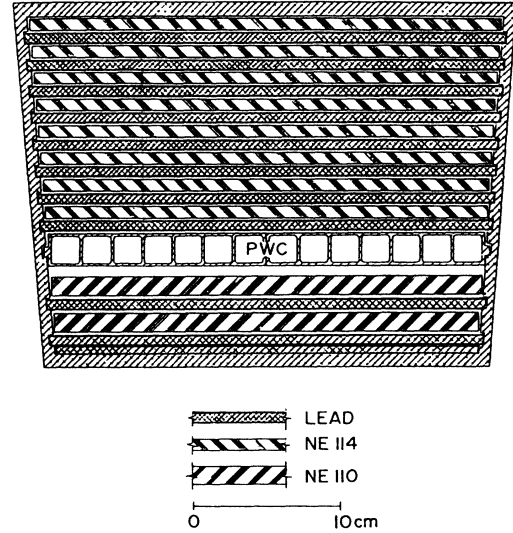
FIG. 2. Cross section through a barrel shower-counter module.
