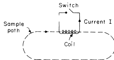
FIG. 2. Sample path through the superconducting loop used for magnetic-charge measurement.
